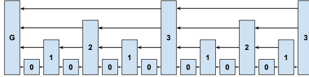
Fig. 3. The probabilistic hierarchical blockchain. Higher levels have achieved a higher difficulty during mining. All blocks are connected to the genesis block G .
