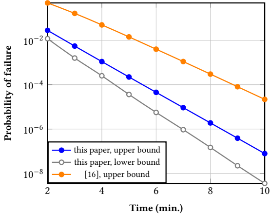
Figure 2: Our upper and lower bounds on settlement failure probability for Ethereum with a 10% adversary and 2 second network delays; results from [16] included for comparison.
