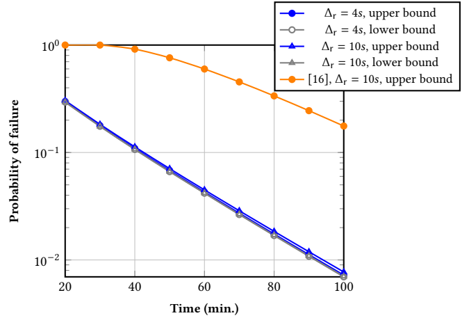
Figure 4: Bitcoin temporal settlement failure for a 10% adversary, results from [16] for comparison.
