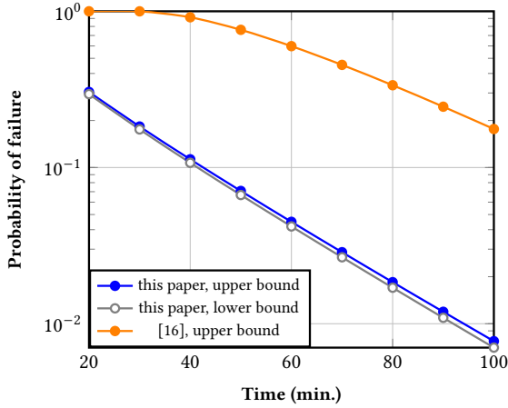
Figure 1: Our upper and lower bounds on settlement failure probability for Bitcoin with a 10% adversary and 10 second network delays; results from [16] included for comparison
