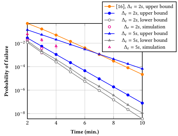
Figure 5: Ethereum temporal settlement failure for a 10% adversary, results from [16] for comparison.
