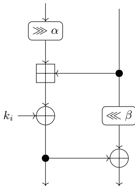
Fig. 7: One round of Speck with round key k_i .
