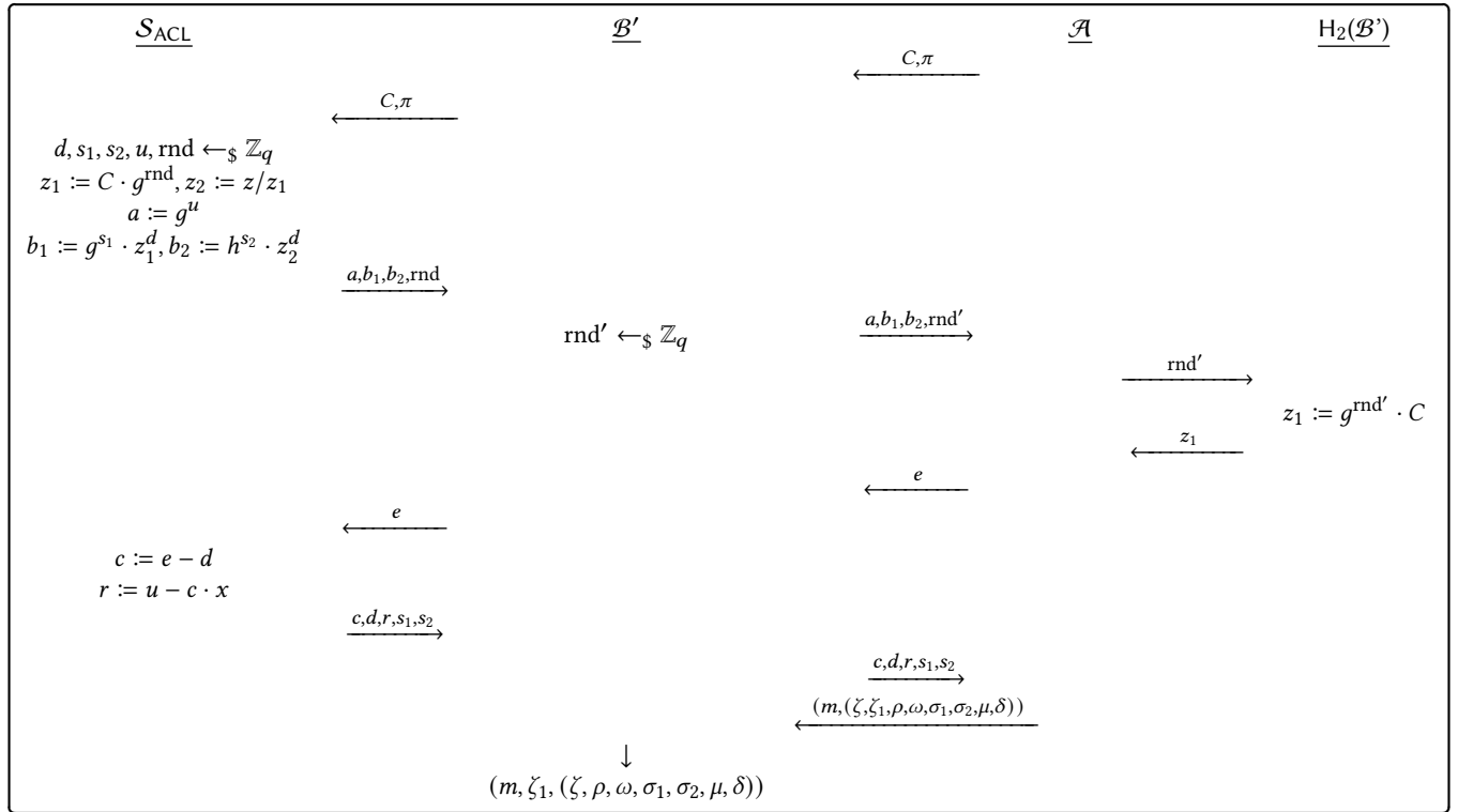
Figure 3: A high-level overview of the reduction \mathcal{B}' . It reduces the OMUF security of ACL to the OMUF security of \text{BS}_{\text{Abe}} . In this figure, S_{\text{ACL}} is the challenger's signer oracle, \mathcal{B}' is the reduction, \mathcal{A} is a forger that wins \ell -OMUF against \text{BS}_{\text{ACL}} , and H_2 is the RO of \text{BS}_{\text{ACL}} , which is simulated by the reduction \mathcal{B}' .
