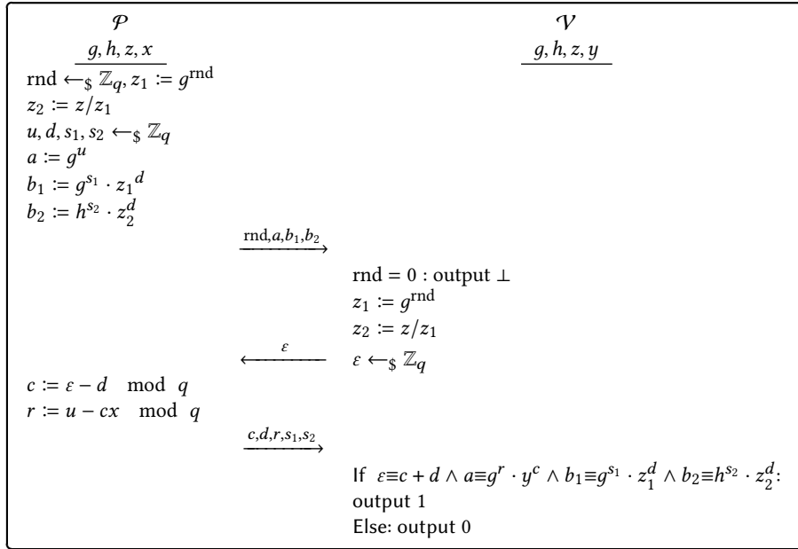
Figure 2: This figure depicts the interaction between the prover and the verifier in the identification scheme \text{ID}_{\text{ACL}} .
