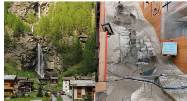
Fig. 2. Left: The cascade of three waterfalls before hitting the village in a moderately inclined, narrow channel. Right: Experiment with corresponding protection measure – a wall with lateral discharge channel to bypass the village.
