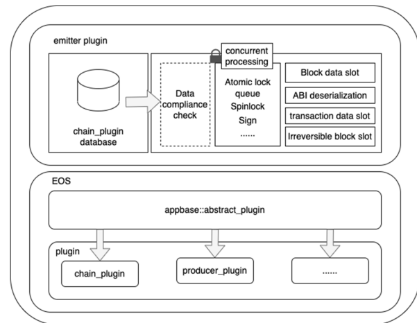
Fig. 5 Data Collaboration
