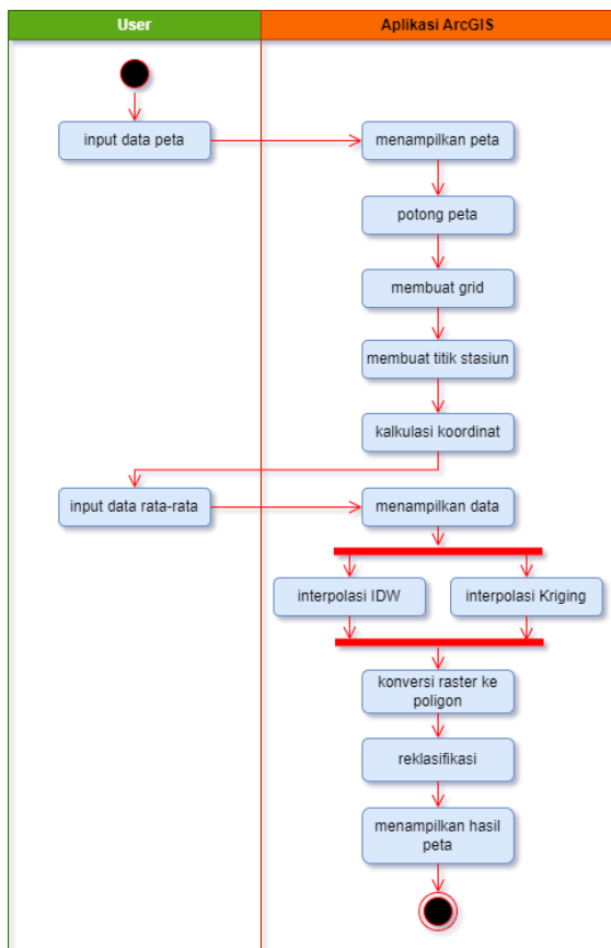
Gambar 3. Activity Diagram
