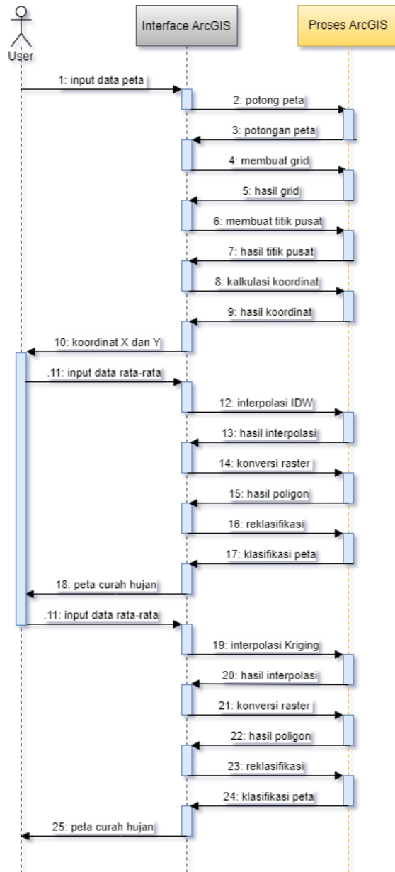
Gambar 4. Sequence Diagram
