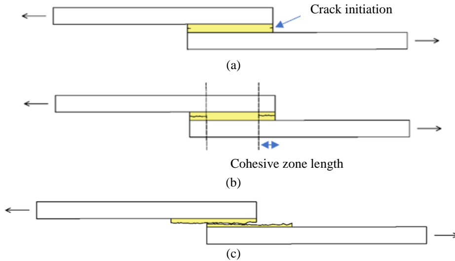
Fig. 6 - Sketch of damage plot at key-points labelled in Fig. 5(a)
