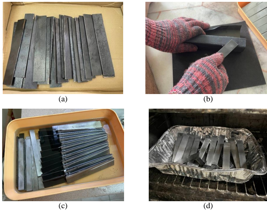
Fig. 1 - Surface preparation of adherend prior to mechanical testing; (a) low carbon steel ready for surface treatment; (b) sanding process using 120 grit size sandpaper; (c) immersed in acetone solution to eliminate impurities; (d) oven-heated under 120°C
