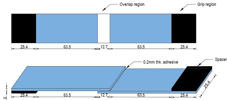
Fig. 3 - Dimensions of single-lap joint configurations according to ASTM D1002
