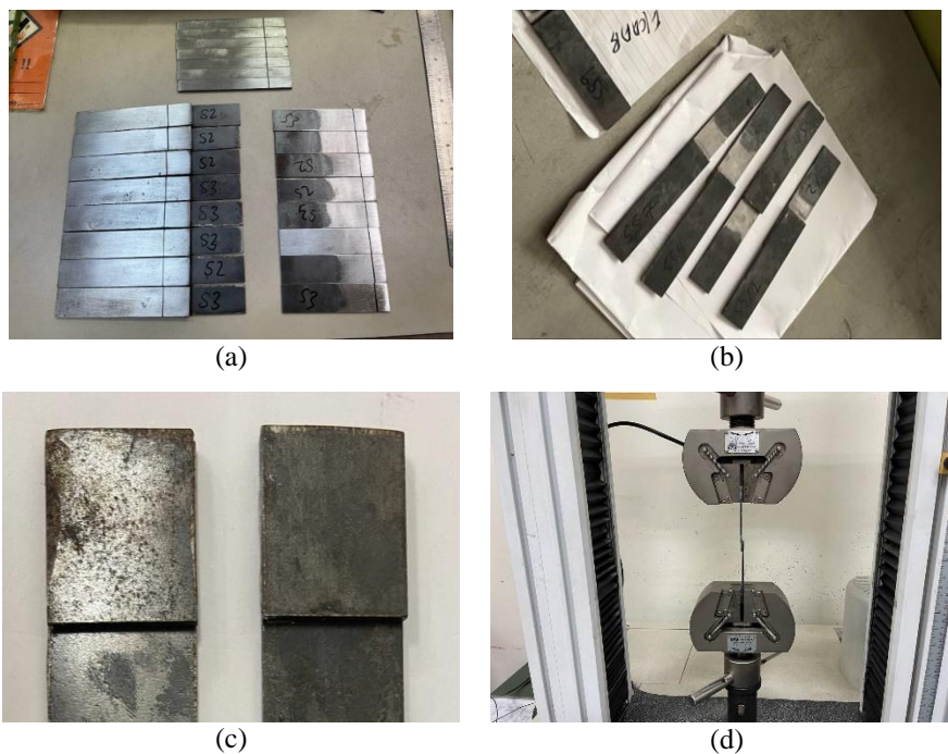
Fig. 4 - Experimental procedures in the single-lap shear test; (a) lines drawn to indicate overlap region; (b) SLJ bonding using TEEP; (c) providing spacers to avoid primary bonding; (d) single-lap shear test set-up
