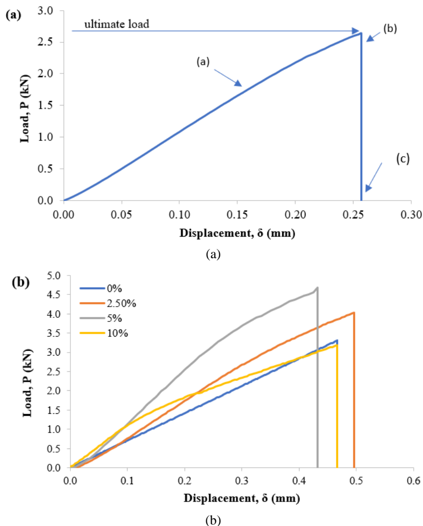
Fig. 5 - Load-displacement profile; (a) typical load-displacement of single-lap joint; (b) load-displacement with different incorporation of TEEP volume fractions
