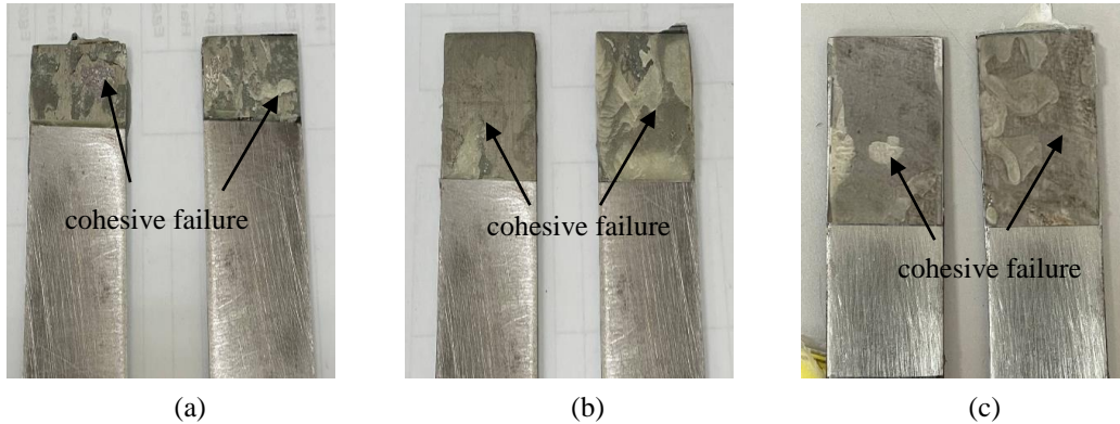
Fig. 7 - Cohesive failure in different adhesive overlap length; (a) 12.7 mm; (b) 25.4 mm; (c) 38.1 mm
