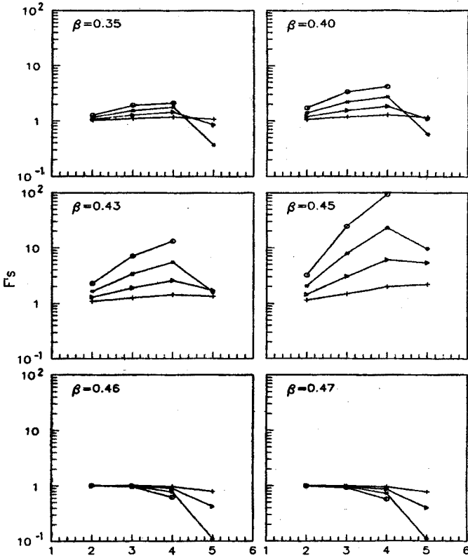
Fig. 1. Monte Carlo results for the factorial moments: F^{(i)} , i = 2(+) , 3(\Delta) , 4(*) , 5(\circ) ; as the function of the cell size, and for various temperatures T = \frac{1}{3}
