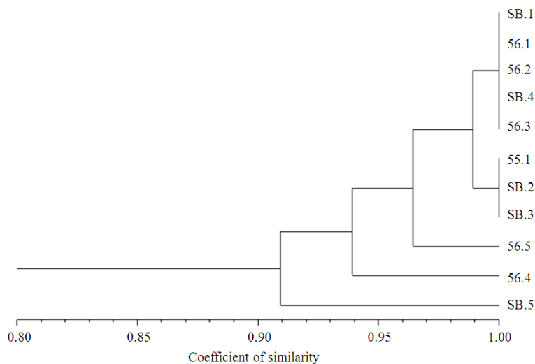
Fig. 3. Similarity of carbon utilization of cultured Streptomyces microorganisms from the Laguna Madre. A total of 95 carbon sources were tested using BIOLOG™ plates. Based on the number of positive tests and which tests were positive, a carbon utilization profile was created and compared to the profile of all other tested isolates. The similarity coefficient is shown on the x-axis
