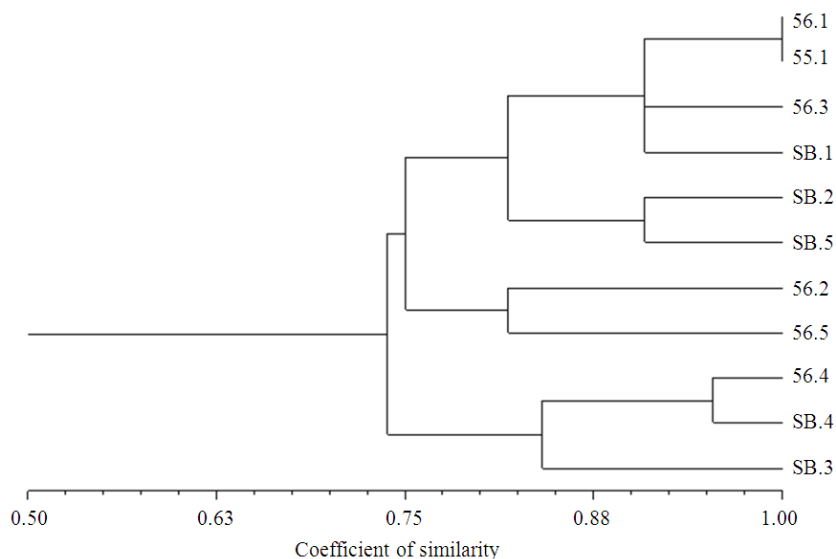
Fig. 2. Similarity of cultured Streptomyces microorganisms from the Laguna Madre based on API 20E ® phenotype profiles. A total of 22 different enzymatic reactions were assayed using API 20E ® strips. Based on the number of positive tests and which of the 22 tests were positive, a phenotype profile was created and compared to the profile of all other tested isolates. The similarity coefficient is shown on the x-axis
