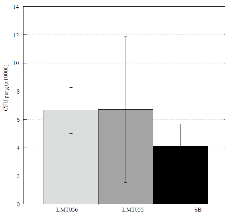
Fig. 1. Estimated density of bacteria in Laguna Madre sediment samples collected in June 2006. Sediment was diluted and spread on Marine 2216 agar. Values are reported as colony forming units per gram (cfu per gram \times 10,000 ) wet sediment. Shown are the means of triplicate incubations with standard deviation
