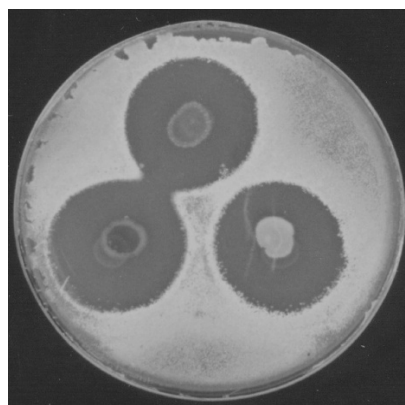
Fig. 4. Representative interference competition plate showing zones of inhibited growth
