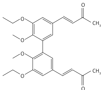
Figure 7. (3E,3'E)-4,4'-(5,5'-diethoxy-6,6'-dimethoxy-[1,1'-biphenyl]-3,3'-diyl)bis(but-3-en-2-one) (15)
