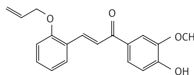
Figure 15. (E)-3-(2-(allyloxy)phenyl)-1-(4-hydroxy-3-methoxyphenyl)prop-2-en-1-one (28)
