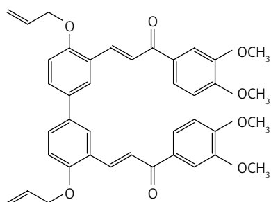
Figure 18. (2E,2'E)-3,3'-(4,4'-bis(allyloxy)-[1,1'-biphenyl]-3,3'-diyl)bis(1-(3,4-dimethoxyphenyl)prop-2-en-1-one) (31)
