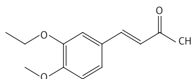
Figure 6. (E)-4-(3-ethoxy-4-methoxyphenyl)but-3-en-2-one (14)
