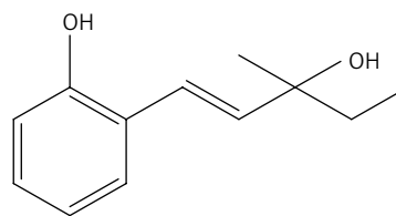
Figure 13. (E)-2-(3-hydroxy-3-methylpent-1-en-1-yl)phenol (26)
