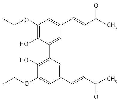
Figure 5. (3E,3'E)-4,4'-(5,5'-diethoxy-6,6'-dihydroxy-[1,1'-biphenyl]-3,3'-diyl)bis(but-3-en-2-one) (13)
