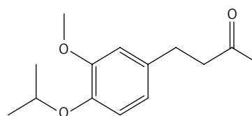
Figure 23. 4-(4-isopropoxy-3-methoxyphenyl)butan-2-one (38)
