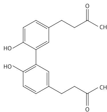
Figure 11. 4,4'-(6,6'-dihydroxy-[1,1'-biphenyl]-3,3'-diyl)bis(butan-2-one) (23)
