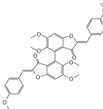
Figure 2. (2Z,2'Z)-5,5',6,6'-tetramethoxy-2,2'-bis(4-methoxybenzylidene)-[4,4'-bibenzofuran]-3,3'(2H,2'H)-dione (2)
