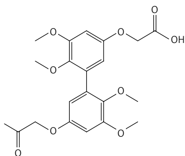
Figure 21. 2,2'-((5,5',6,6'-tetramethoxy-[1,1'-biphenyl]-3,3'-diyl)bis(oxy))diacetic acid (44)
