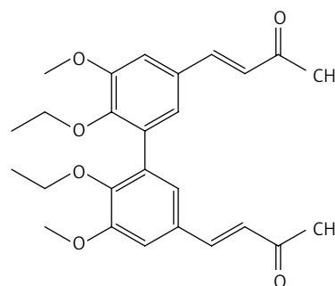
Figure 8. (3E,3'E)-4,4'-(6,6'-diethoxy-5,5'-dimethoxy-[1,1'-biphenyl]-3,3'-diyl)bis(but-3-en-2-one) (17)
