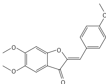
Figure 1. (Z)-5,6-dimethoxy-2-(4-methoxybenzylidene)benzofuran-3(2H)-one (1)
