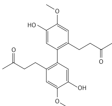
Figure 3. 4,4'-(5,5'-dihydroxy-4,4'-dimethoxy-[1,1'-biphenyl]-2,2'-diyl)bis(butan-2-one) (5)
