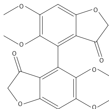
Figure 22. 5,5',6,6'-tetramethoxy-[4,4'-bibenzofuran]-3,3'(2H,2'H)-dione (37)
