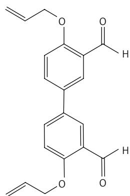
Figure 10. 4,4'-bis(allyloxy)-[1,1'-biphenyl]-3,3'-dicarbaldehyde (40)
