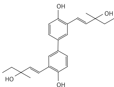
Figure 14. 3,3'-bis((E)-3-hydroxy-3-methylpent-1-en-1-yl)-[1,1''-biphenyl]-4,4'-diol (27)
