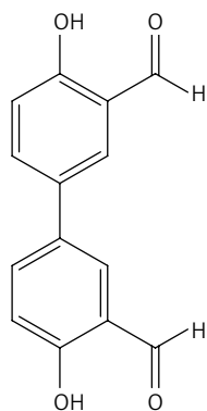
Figure 12. 4,4'-dihydroxy-[1,1''-biphenyl]-3,3'-dicarbaldehyde (25)
