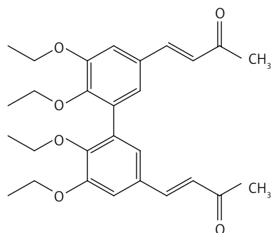
Figure 9. (3E,3'E)-4,4'-(5,5',6,6'-tetraethoxy-[1,1'-biphenyl]-3,3'-diyl)bis(but-3-en-2-one) (19)
