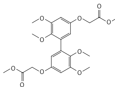
Figure 20. Dimethyl 2,2'-((5,5',6,6'-tetramethoxy-[1,1'-biphenyl]-3,3'-diyl)bis(oxy))diacetate (43)
