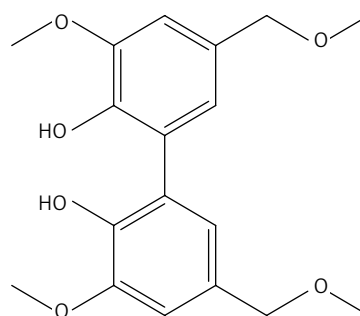
Figure 4. 3,3'-dimethoxy-5,5'-bis(methoxymethyl)-[1,1'-biphenyl]-2,2'-diol (11)
