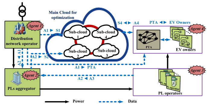
Fig. 1. The agent-based structure of the proposed framework.
