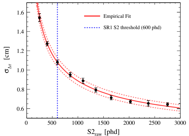
FIG. 10. Dependence of the radial position resolution of the wall events on S2 pulse size. Events below the ER band and in the WS sideband region ( 80 < S1c < 500 \text{ phd} ) were selected to determine the radial position resolution of wall events, and were observed to depend on the S2 pulse size based on the equation: \sigma_{\Delta r}(S2) = \frac{a}{\sqrt{S2}} + b , where the fitting parameters a and b were 21.04 \pm 0.65 and 0.22 \pm 0.02 , respectively.
