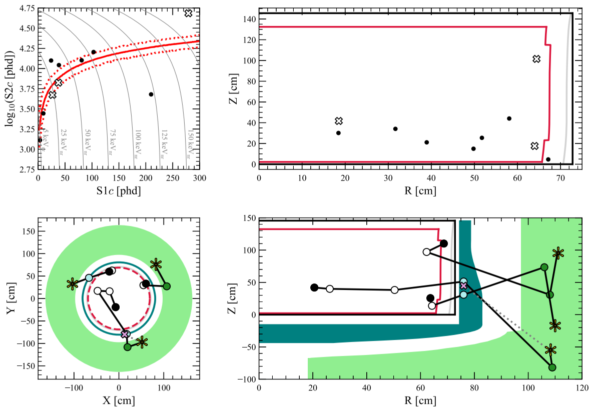
FIG. 9. Locations of MS neutron events identified in the SR1 dataset, correlated across all three detectors. Top : Distribution of the 10 identified neutron events in \log_{10}(S2c) - S1c space overlaid with the MS NR band, as well as their averaged positions in the TPC. White crosses denote three example events displayed in detail on the second row. Bottom : Chains of reconstructed scatters demonstrating interdetector coincidences in tagging neutron events. Working outwards: the red outline indicates the SR1 FV; the gray curve highlights the TPC wall boundary in reconstructed space; the black box indicates the physical edges of the active xenon volume; the teal profile denotes the liquid xenon Skin; the outermost green region represents the OD acrylic tanks containing the GdLS. As the exact chronology of the event could not be determined, interactions were ordered by drift time. Black circles denote the locations of the scatters with shortest drift time in the given neutron MS chain, with empty circles showing the positions of other interactions in the TPC. Scatters in the Skin and OD are shaded in blue and green respectively. Neutron captures in the OD are marked as a *, and resulting gamma-ray splashes observed in the Skin are labeled with a pink cross. OD points are randomly assigned radial positions as XY reconstruction there is often biased towards the centre, a correction for which is under development.
