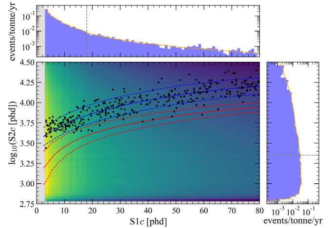
FIG. 12. The accidentals PDF normalized to events/tonne/yr. The 10% and 90% quantiles (dashed) as well as the median (solid) of the ER and NR bands, as reported in Ref. [7], are shown in blue and red, respectively. SR1 WS events remaining after all data selections are also shown (black dots). The regions outside the WS ROI are marked with a shaded gray area. The number of predicted accidental events in the entire ROI is 1.2 (0.2 inside the NR band). The top and right panels show the projections on each axis of the ACS events surviving all analysis cuts, where the distribution falls off at small \log_{10}(S2c) due to the applied 600 phd lower bound in raw S2 pulse size. The orange lines represent the functions that were used to build the two-dimensional PDF. Regions with larger data fluctuations, starting from the dashed gray lines, were smoothed out.
