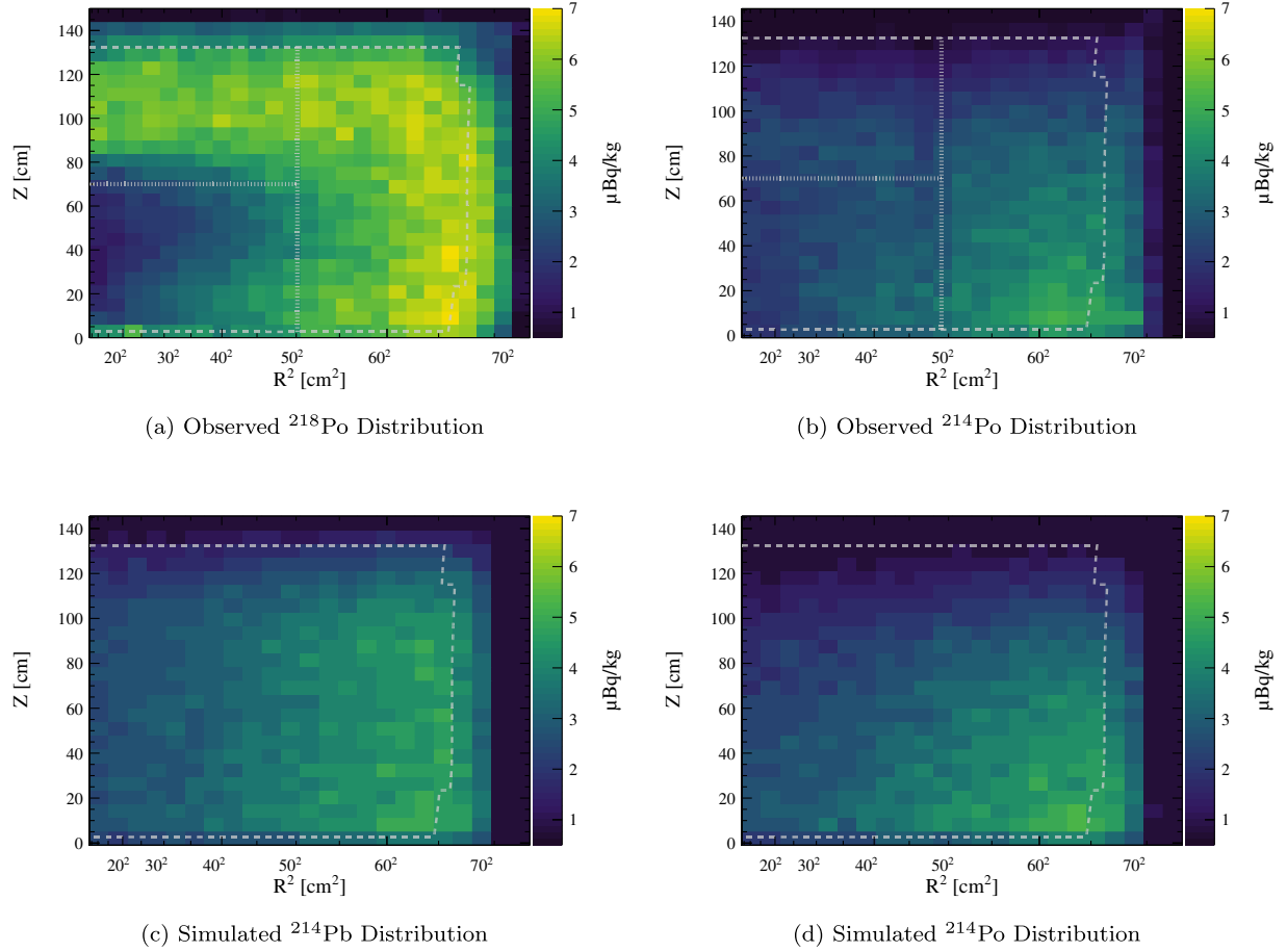
FIG. 2. The observed and simulated distributions of selected ^{222}\text{Rn} daughters. The ^{218}\text{Po} distribution in data was found from SS events and is shown in panel (a); the ^{222}\text{Rn} distribution can be considered to be nearly identical to that of ^{218}\text{Po} . The measured ^{214}\text{Po} distribution is shown in panel (b), for which the S1-S2 pair of ^{214}\text{Po} was extracted from each Bi-Po event to reconstruct its position analogously to a SS event. Simulated ^{214}\text{Pb} and ^{214}\text{Po} distributions in panels (c) and (d), respectively. The robustness of the toy model was validated from the agreement between the simulated and observed ^{214}\text{Po} distributions. The FV boundary is shown with a dashed gray line on all panels, whereas for the observed distributions, two additional dotted lines further separate the FV into upper, lower, and outer regions. These volumes are used in Table I to quantify the nonuniformity of the observed alphas.
