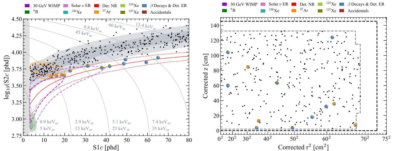
FIG. 15. Left : Low-energy data after all data quality and physics cuts in \log_{10}(S2c) - S1c space. Contours enclose 1\sigma and 2\sigma of the best-fit background model (shaded gray), the ^{37}\text{Ar} component (orange ellipses), a 30 GeV/c 2 WIMP (purple dashed lines), and ^8\text{B} solar neutrinos (shaded green regions). The solid red line shows the NR median, and the red dotted lines indicate the 10% and 90% quantiles. Right : Corrected z and r^2 positions of the same data. Dashed black lines outline the active liquid xenon volume and dashed gray lines represent the fiducial volume. In both figures, events falling below the 2\sigma contour of the best-fit background model are shown as pie charts for which the size of each wedge is determined by the relative weight of each of the background components in the fit.
