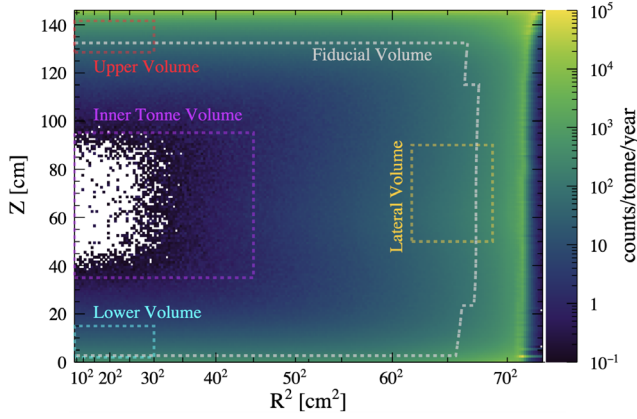
FIG. 6. The simulated position distribution of all single scatter ER events from detector components and cavern gamma rays. Overlaid are the three subvolumes (upper, lateral, lower) and the SR1 FV in which fits were performed. The inner one-tonne volume, used for the fitting of internal sources in Sec. III C, is also shown.
