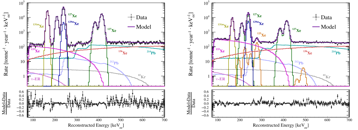
FIG. 4. Fit results for the SR1 exposure for the inner one-tonne region of the TPC. Data are shown in black and the summed background model in purple. Left : Pre-DD calibrations Right : Post-DD calibrations.
