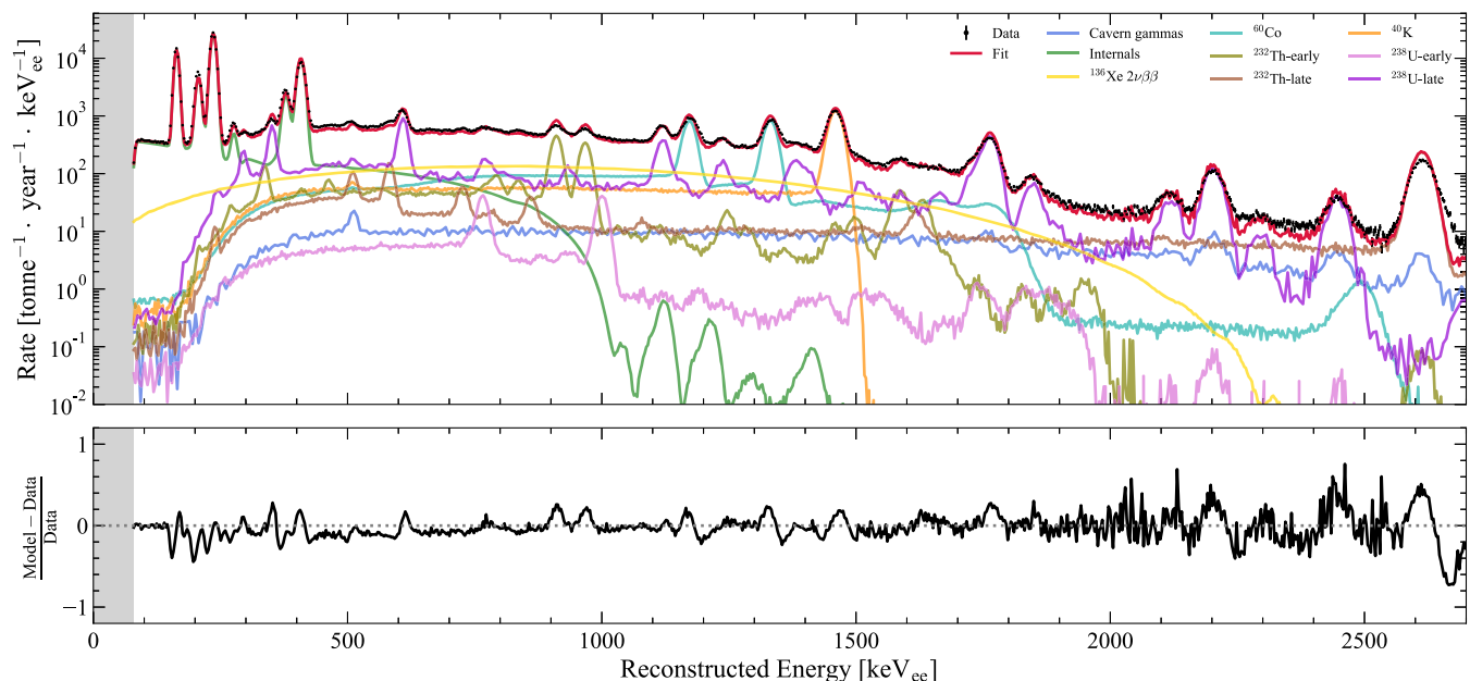
FIG. 7. Fitted detector component spectra in the SR1 FV, following the prescribed sequence of subvolume fits. The fit results are consistent with an average residual of approximately zero, with fluctuations at certain peaks arising from imperfections in energy resolution matching between data and simulations. The contribution from internals is fixed here according to the outputs of the central subvolume fit. Gray shading is used to obscure data < 80 \text{ keV}_{\text{ee}} to avoid inferences in the regions of interest for future EFT and ^{124}\text{Xe} 2\nu\text{DEC} searches.
