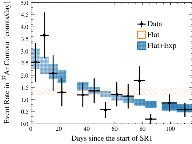
FIG. 11. Time dependence of events in the 2\sigma contour for ^{37}\text{Ar} in \log_{10}(\text{S}2c)\text{-S}1c space (see Fig. 15). Black points show the data. The orange band shows the best fit to a rate constant in time, including systematic uncertainty from the fit, and the blue band shows the best fit to a rate constant in time plus an exponential decay with a 35 day half-life. The data and predictions are corrected for the live time in each bin.
