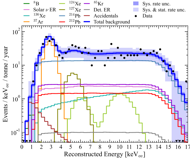
FIG. 14. Background model before fitting to the SR1 data (except for the ^{37}\text{Ar} component, for which the post-fit normalization is used). The total model is shown in dark blue, and SR1 data after all WS cuts have been applied are denoted by the black points. This represents a background event rate of (6.3 \pm 0.5) \times 10^{-5} events/keV _{ee} /kg/day.
