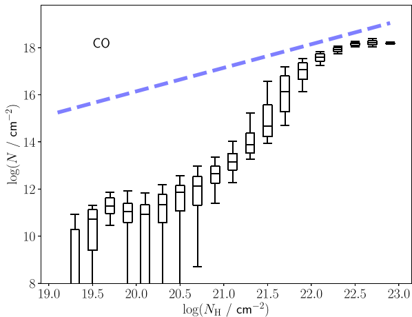
Figure 8. Box plot of \text{CO} column density versus N_{\text{H}} . Boxes show the median and the 25th/75th percentiles; whiskers show the 10th and 90th percentiles. The dashed blue line shows the column density expected if all carbon is in the form of \text{CO} .
