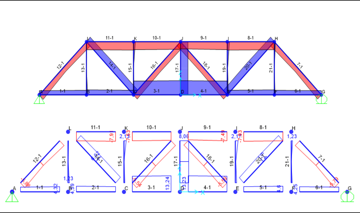
Figure 30 Stress results from SAP 2D static load of 125N at joint D
