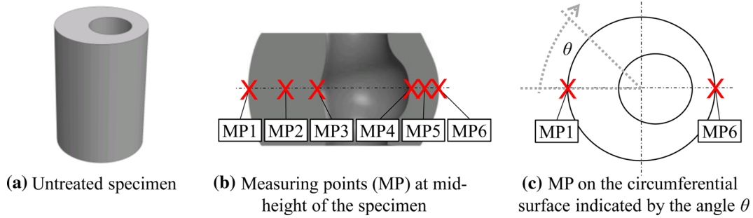
Fig. 6 Illustration of the untreated specimen (a), the measuring points MP1 to MP6 at mid-height of the specimen (b) as well as the angle \theta on the circumferential surface of the specimen (c)
