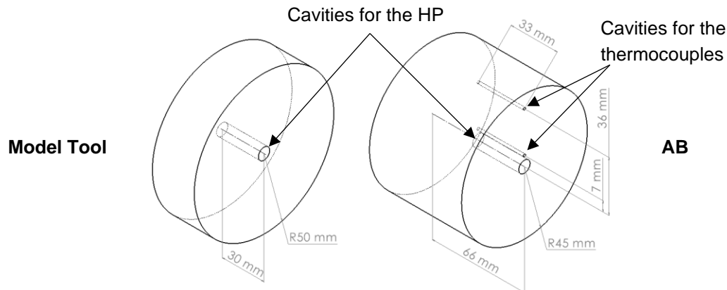
Figure 2 Basic dimensions of the model tools (left) and the AB (right)
