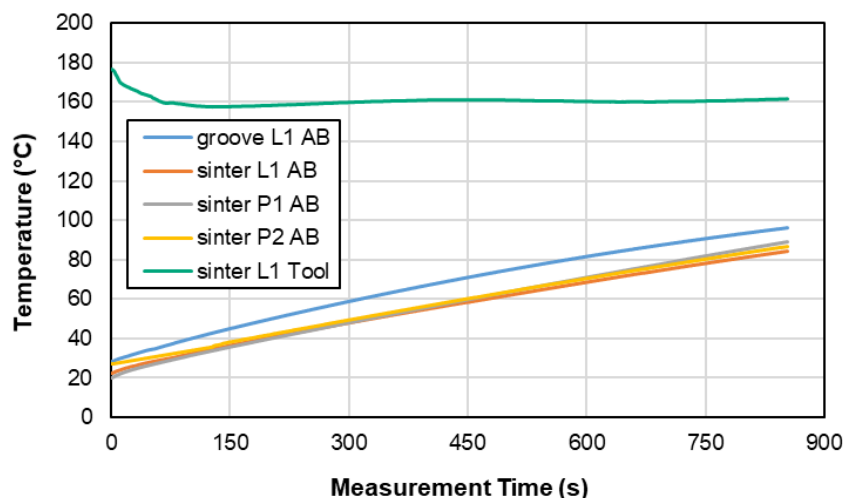
Figure 4 Averaged temperature curves over time of the AB with different fitting designs, exemplary temperature curve of the tool with sintered L1
