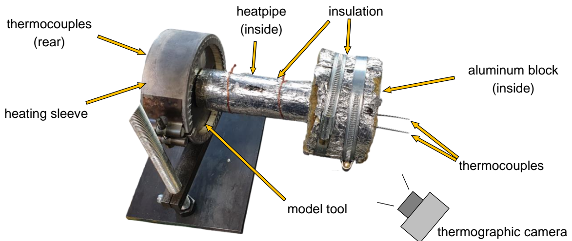
Figure 1 Experimental setup for heat transfer measurements
