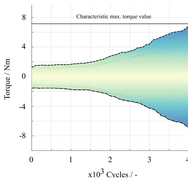
Fig. 2 Measured torque signal reduced by the moment of inertia of the moving components for a test at f=3 Hz, \Theta=7^\circ . The black dashed lines show the development of the maximum and minimum torque. The solid black line marks the maximum torque value that was reached during the test [16]
