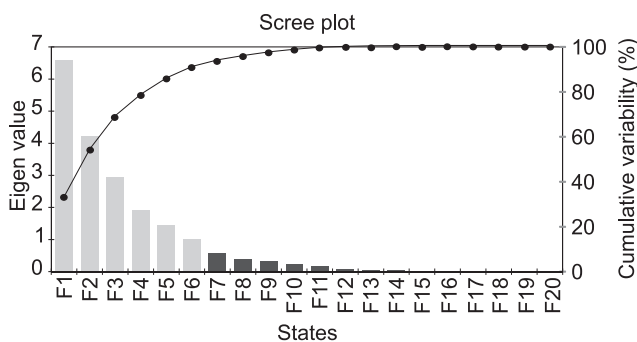
Fig. 1. Scree plot of eigen value and cumulative variability.
