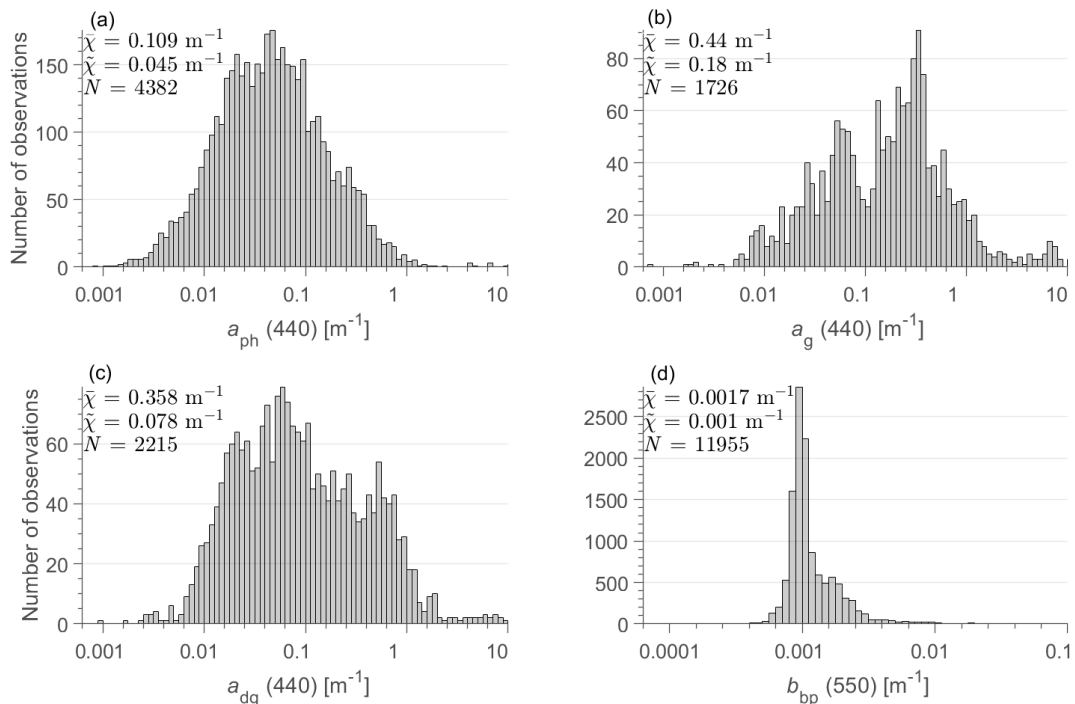
Figure 2. Histograms and relevant statistical parameters of field measurements of (a) a_{\text{ph}}(440) , (b) a_{\text{g}}(440) , (c) a_{\text{dg}}(440) , and (d) b_{\text{bp}}(550) . N is the number of measurements, and \bar{x} and \tilde{x} are the mean and median values of each IOP, respectively.
