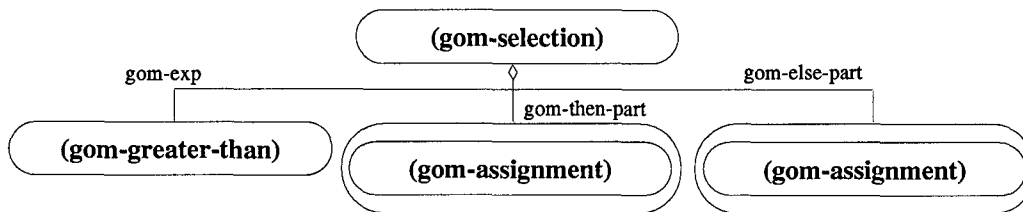
Figure 69 GOM Selective Control Flow Example
