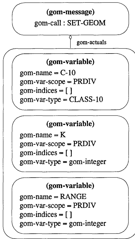
Figure 81 GEM Attribute Array Access Object
