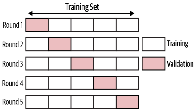
Figure 3: K-Fold cross validation when K=5.
