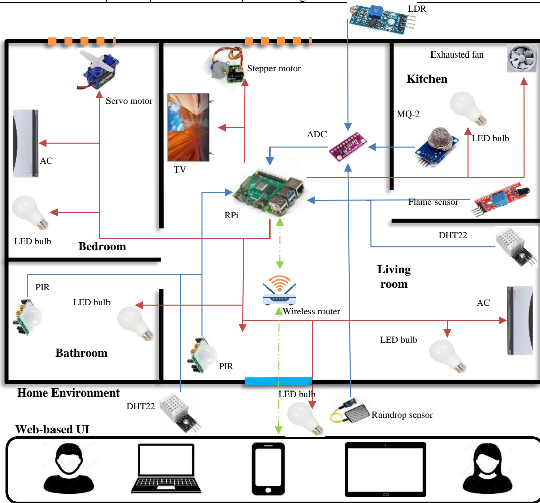
Figure 5: Home architecture and connected sensors, and appliances (red lines indicates wired RPi output, blue lines indicate wired RPi input, and the green lines refers to wireless communication).
