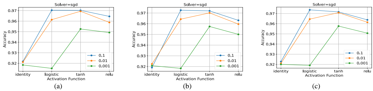
Figure 17: MLP performance with different K-Folds. (a) K-Fold=3. (b) K-Fold=5. (c) K-Fold=10.
