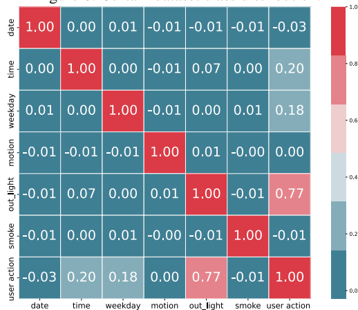
Figure 7: Curtain dataset column correlations.
