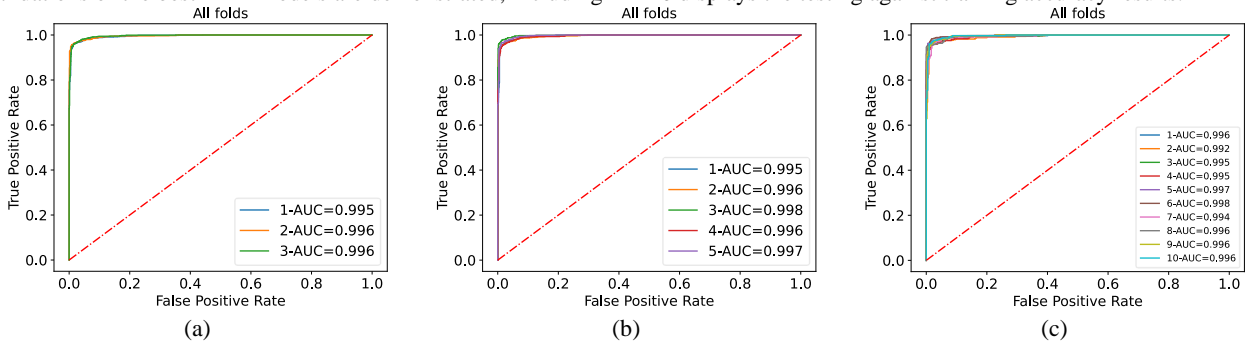
Figure 19: ROC curve with AUC results for MLP classifier. (a) K-Fold=3. (b) K-Fold=5. (c) K-Fold=10.
