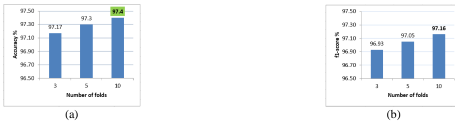
Figure 10: DT performance with different K-Folds. (a) Accuracy score. (b) F1-score.
