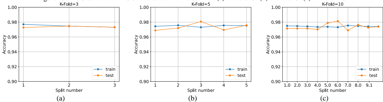
Figure 20: Model performance for MLP classifier (Train vs Test accuracy). (a) K-Fold=3. (b) K-Fold=5. (c) K-Fold=10.
