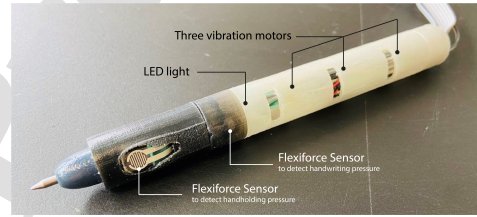
Figure 29: ApEn: the stress-aware pen.
