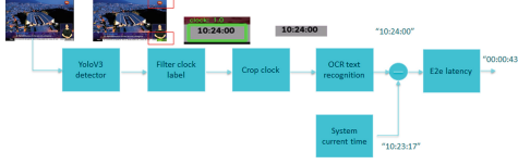
Figure 7: Architecture approach for live streaming latency estimation.
