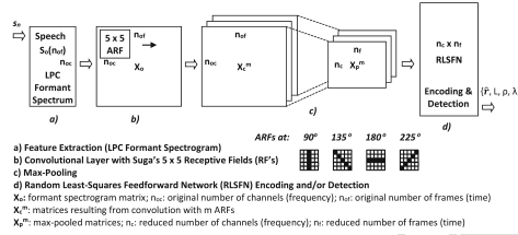
Figure 27: Architecture of the CNN proposed in [194].
