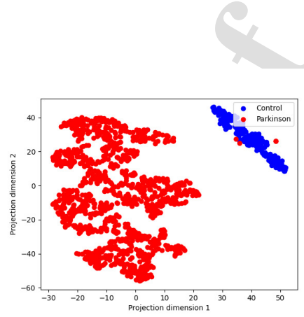
Figure 26: Projection over the first two dimensions of the embeddings associated with controls (blue) and PD (red).
