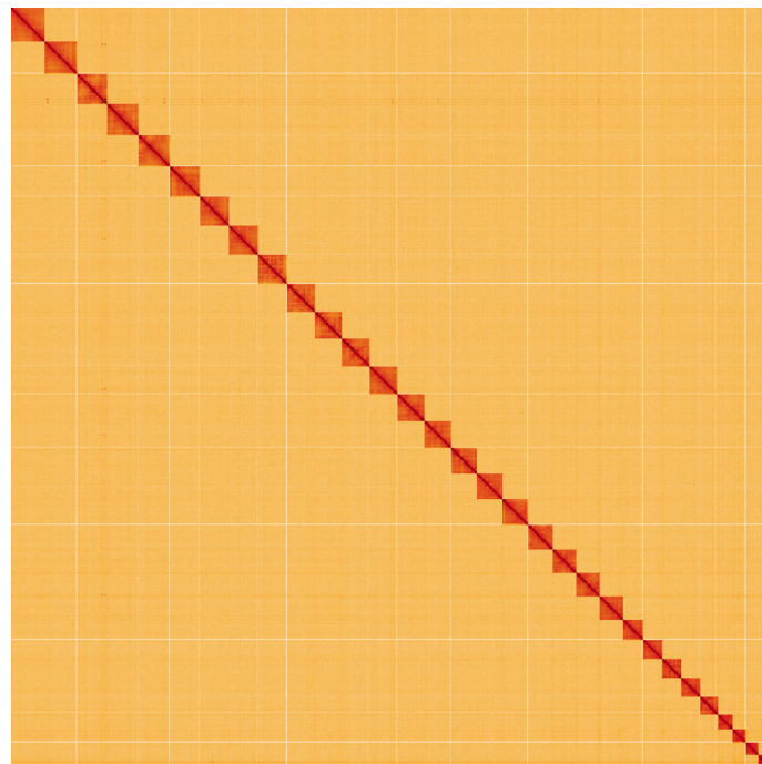
Figure 5. Genome assembly of Ptilodon capucinus , ilPtiCapc1.1 alternate haplotype: Hi-C contact map of the ilPtiCapc1.1 alternate haplotype assembly, visualised using HiGlass. Chromosomes are shown in order of size from left to right and top to bottom. An interactive version of this figure may be viewed at https://genome-note-higlass.tol.sanger.ac.uk/1/?d=BqET2dZSTnSs7zhjHqvgWg .
