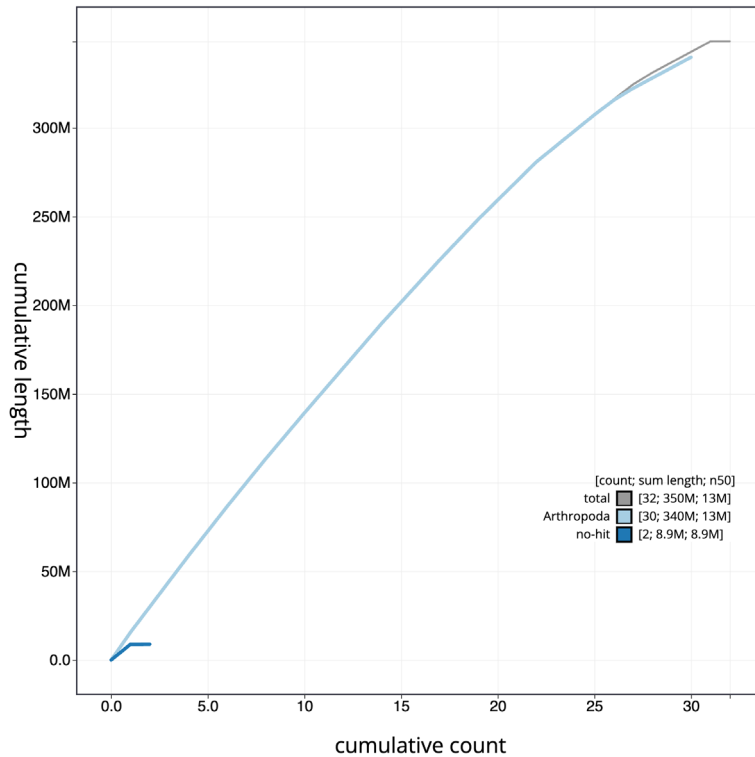
Figure 4. Genome assembly of Ptilodon capucinus , ilPtiCapc1.1: BlobToolKit cumulative sequence plot. The grey line shows cumulative length for all scaffolds. Coloured lines show cumulative lengths of scaffolds assigned to each phylum using the buscogenes taxrule. An interactive version of this figure is available at https://blobtoolkit.genomehubs.org/view/ilPtiCapc1.1/dataset/ilPtiCapc1_1.1/cumulative .
