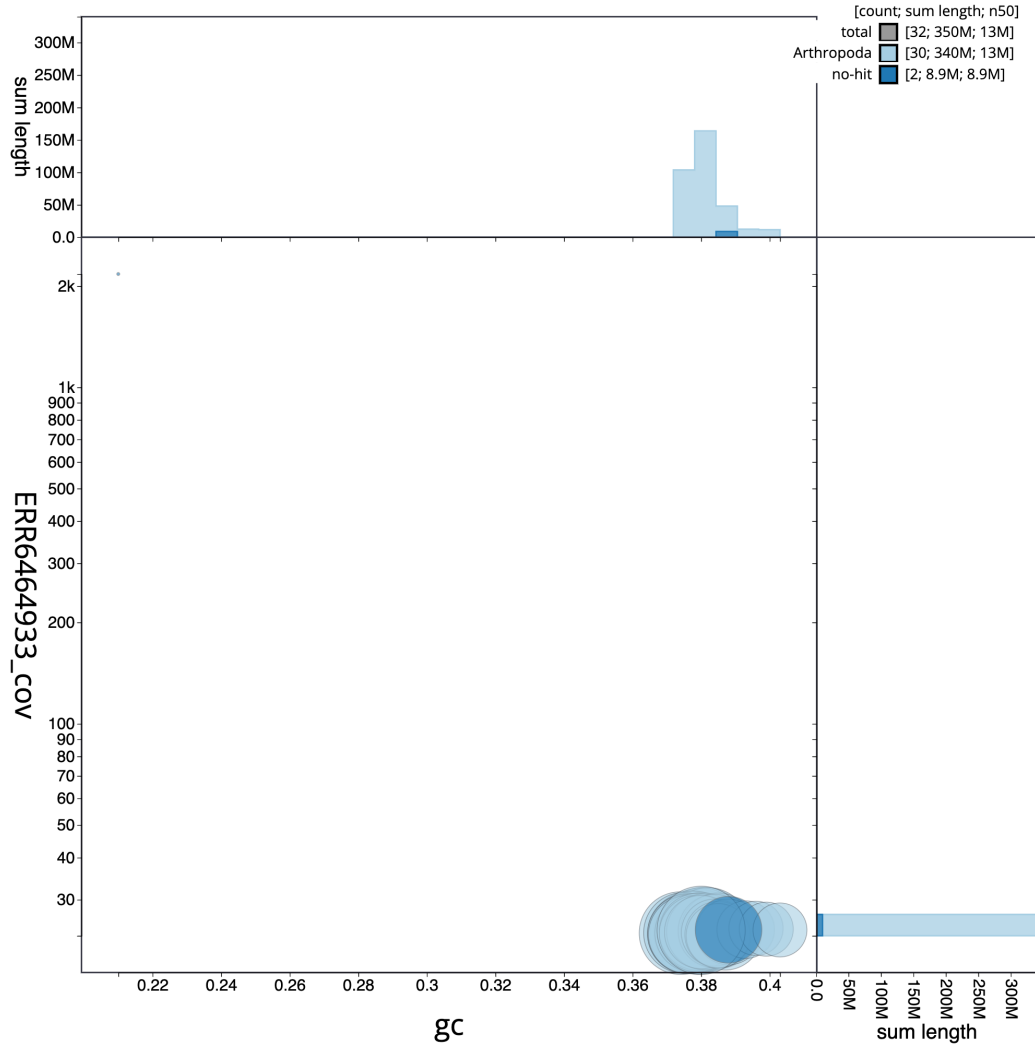
Figure 3. Genome assembly of Ptilodon capucinus , ilPtICap1.1: BlobToolKit GC-coverage plot. Scaffolds are coloured by phylum. Circles are sized in proportion to scaffold length. Histograms show the distribution of scaffold length sum along each axis. An interactive version of this figure is available at https://blobtoolkit.genomehubs.org/view/ilPtICap1.1/dataset/ilPtICap1_1.1/blob .
