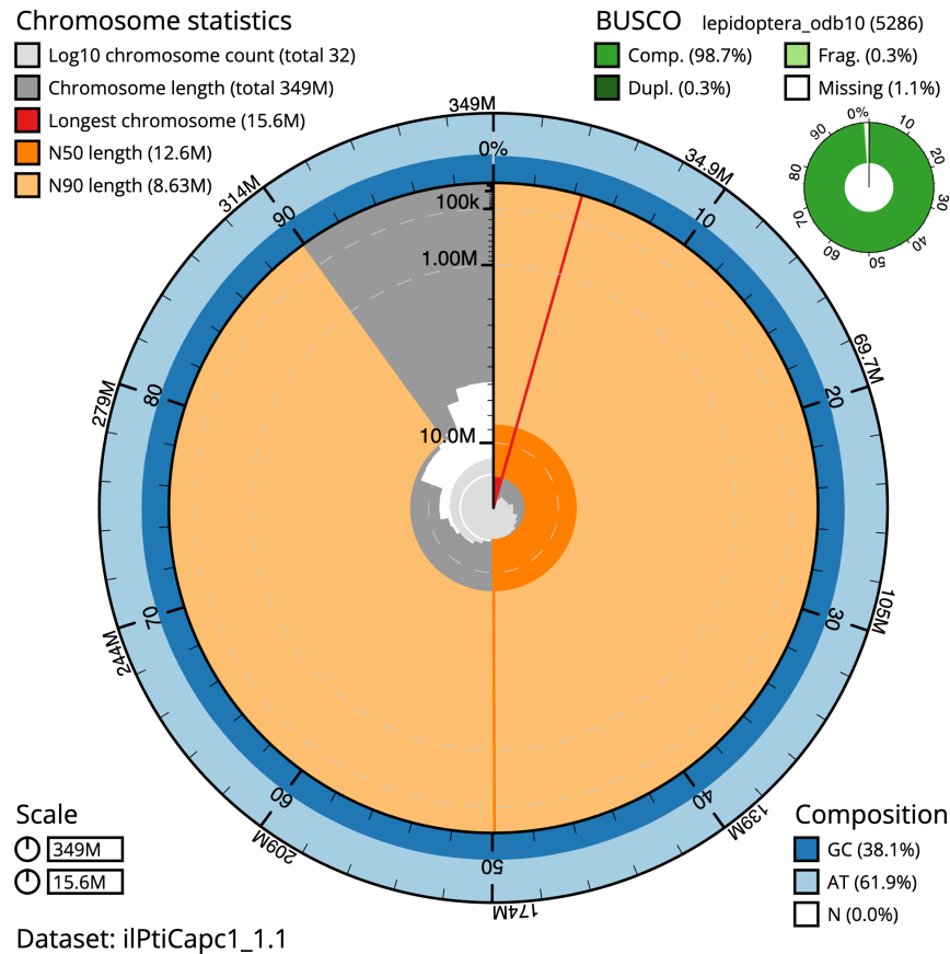
Figure 2. Genome assembly of Ptilodon capucinus , ilPtiCapc1.1: metrics. The BlobToolKit Snailplot shows N50 metrics and BUSCO gene completeness. The main plot is divided into 1,000 size-ordered bins around the circumference with each bin representing 0.1% of the 348,711,871 bp assembly. The distribution of scaffold lengths is shown in dark grey with the plot radius scaled to the longest scaffold present in the assembly (15,614,753 bp, shown in red). Orange and pale-orange arcs show the N50 and N90 scaffold lengths (12,643,213 and 8,629,352 bp), respectively. The pale grey spiral shows the cumulative scaffold count on a log scale with white scale lines showing successive orders of magnitude. The blue and pale-blue area around the outside of the plot shows the distribution of GC, AT and N percentages in the same bins as the inner plot. A summary of complete, fragmented, duplicated and missing BUSCO genes in the lepidoptera_odb10 set is shown in the top right. An interactive version of this figure is available at https://blobtoolkit.genomehubs.org/view/ilPtiCapc1.1/dataset/ilPtiCapc1_1.1/snail .
