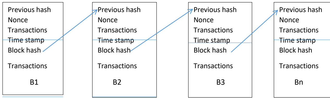
Fig. 1. Blockchain structure[7]
