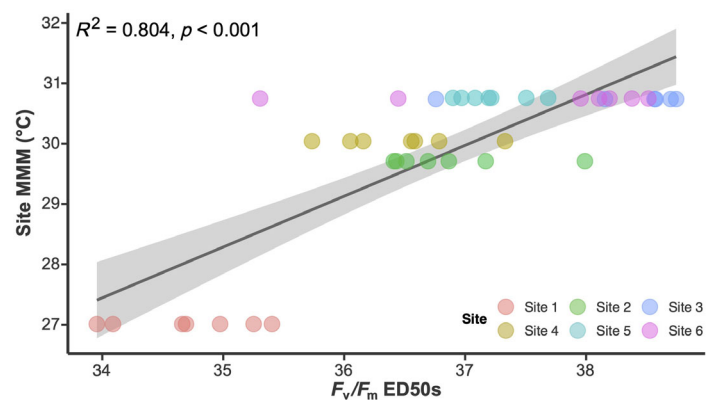
Fig. 5. Correlation between F_v/F_m -based ED50 thermal thresholds and Maximum Monthly Mean (MMM) sea surface temperatures for Stylophora pistillata colonies collected and assayed across six Red Sea reef sites during the summer (6–7 colonies per site, n = 41 ). The black line represents the linear regression, with gray-shaded area indicating the 95% confidence interval.
