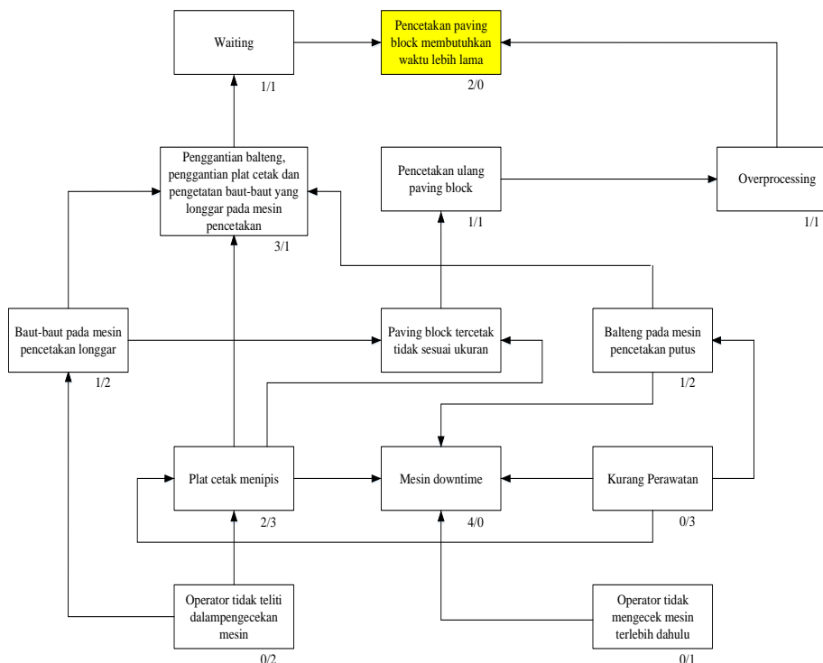
Gambar 4. Relationship Diagram Proses Pencetakan Paving Block
