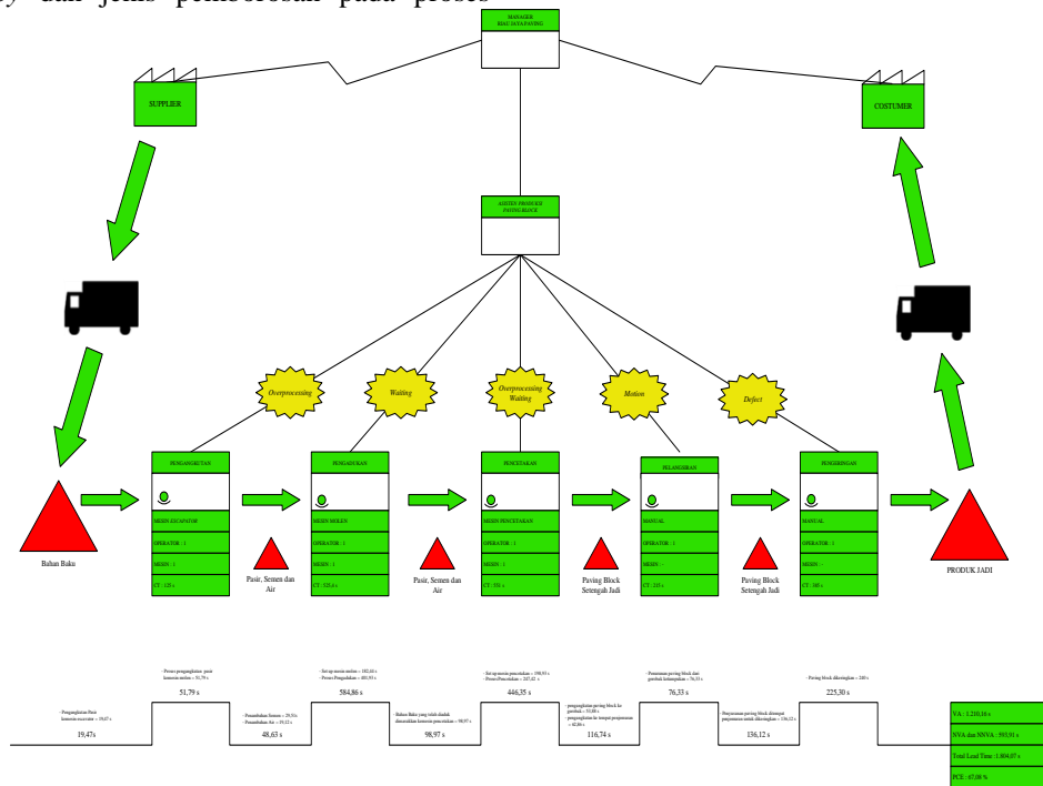
Gambar 2. Current Value Stream Mapping
