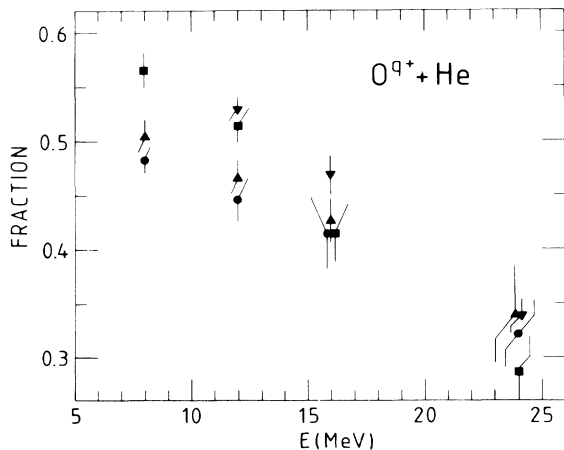
FIG. 1. Fraction of transfer ionization compared to total single-charge transfer, i.e., f = \sigma_{q,q-1}^{02} / (\sigma_{q,q-1}^{01} + \sigma_{q,q-1}^{02}) . The symbols denote charge states as follows: ●, 5+; ▲, 6+; ■, 7+; ▼, 8+.
