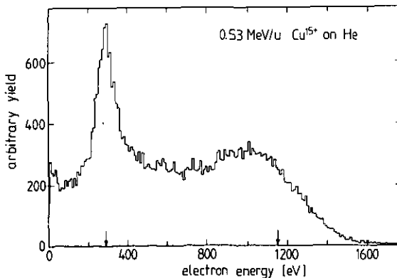
Figure 2. 0° electron spectrum for 0.53 \text{ MeV u}^{-1} \text{ Cu}^{15+} on He. The spectrum is not corrected for the spectrometer transmission function (proportional to 1/E ). The arrows mark the position of the cusp and BE peak (classically calculated).
