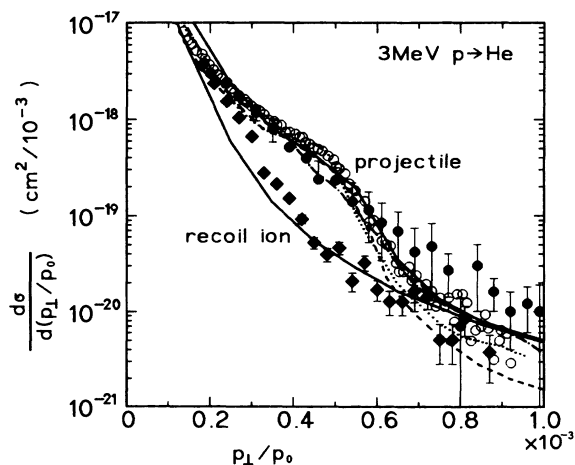
FIG. 1. Differential single-ionization cross sections of He by 3-MeV protons as a function of the transverse momentum transfer to the projectile p_{\text{prol}} ( \bullet , experiment; \circ , experiment Ref. [4]; —, n -CTMC; - · - · -, Born [8]; - - -, Glauber [9]; · · · ·, EDW [10] approximation) and to the recoil ion p_{\text{recl}} ( \blacklozenge , experiment; —, n -CTMC).
