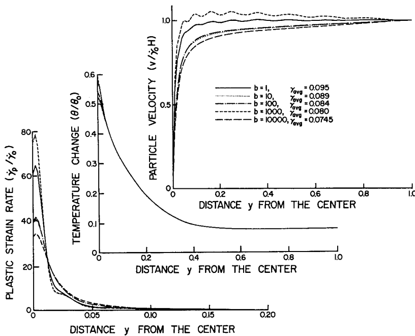
Fig. 2. Effect of the value of material parameter b on the distribution of particle velocity, temperature change and plastic strain rate within the specimen.
