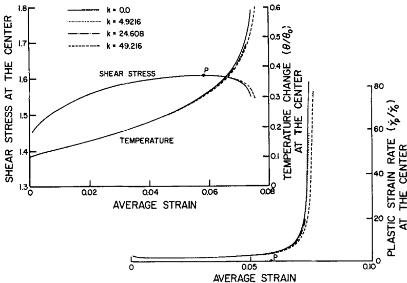
Fig. 9. Effect of the thermal conductivity on the growth of the central shear stress, temperature and the plastic strain rate.
