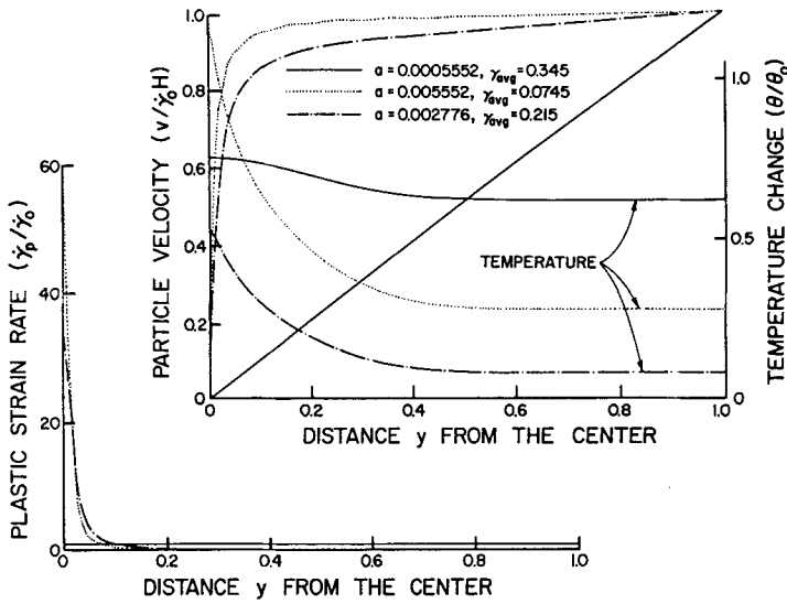
Fig. 8. Variation of the particle velocity, temperature and plastic strain rate within the specimen for different values of \alpha .
