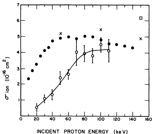
FIG. 5. Total cross sections for ionization of O_2 by protons. \circ : present data; \bullet : de Heer et al. (Ref. 17); \square : Hooper et al. (Ref. 19); \times : Crooks and Rudd (Ref. 18).
