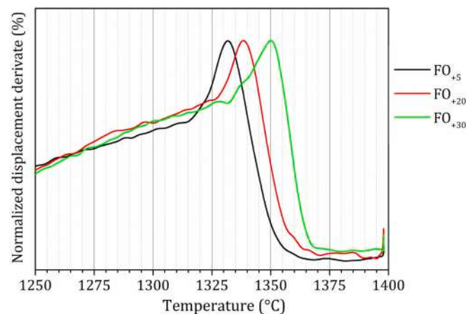
Fig. 5. Normalized displacement derivative curve over the temperature for samples produced with different FOs. The peaks indicate the α-transus temperature, see text.
