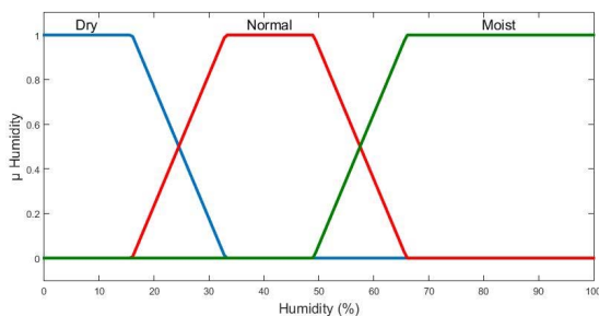
Fig. 2. Membership function of input humidity.
