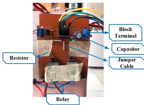
Fig. 8 Relay circuit.
