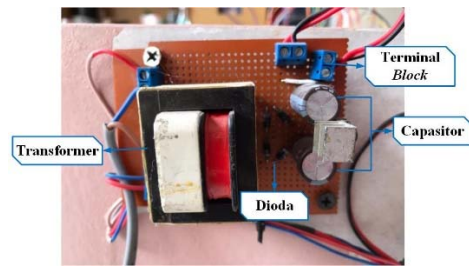
Fig. 7 Power supply circuit.
