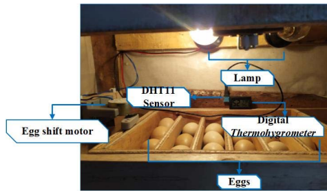
Fig. 6 Inner incubator.
