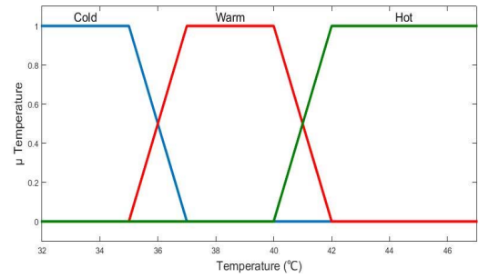
Fig 3. Membership function of input temperature.
