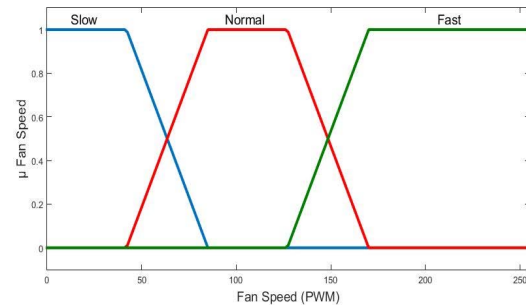
Fig. 4. Membership function of output fan speed
