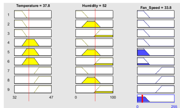
Fig 9. Rule view (optimization/defuzzification results).
