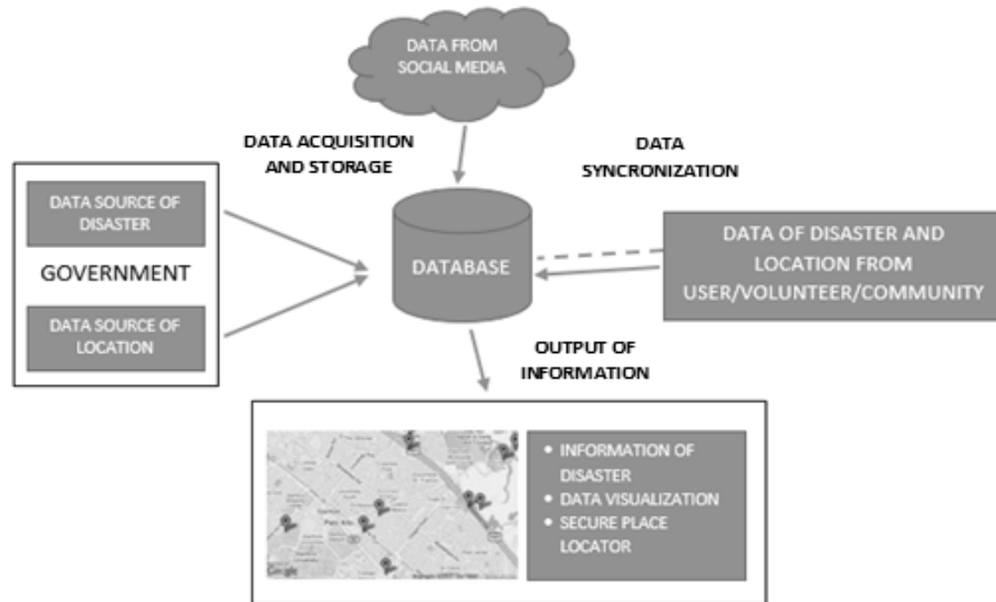
Figure 3. Data and information Circulation in SPL
