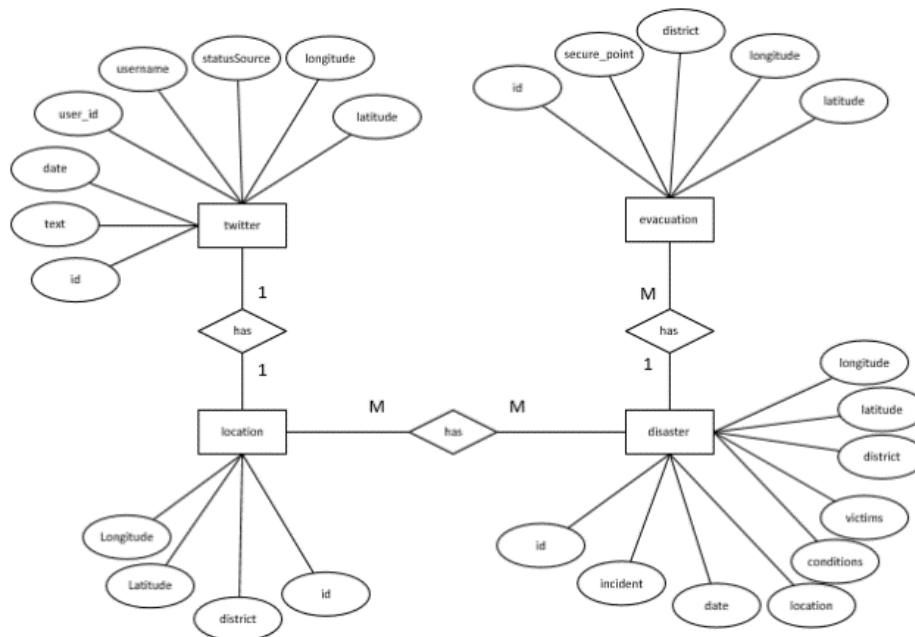
Figure 5. Entity Relationship Diagram for SPL tool
