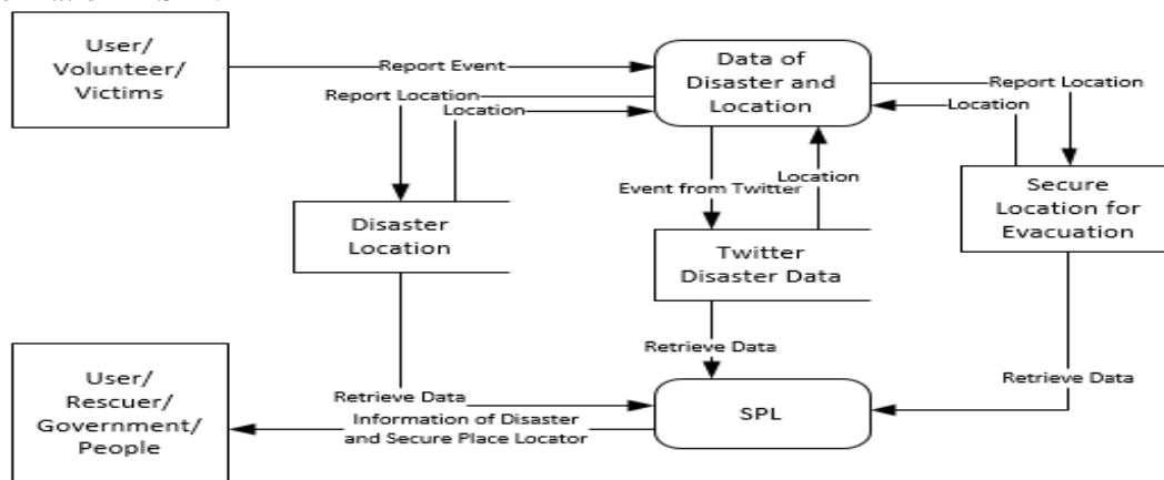
Figure 4. Context Diagram Level 0 in SPL
