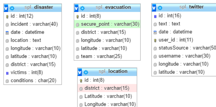
Figure 6. Tables belong to SPL tool in MySQL
