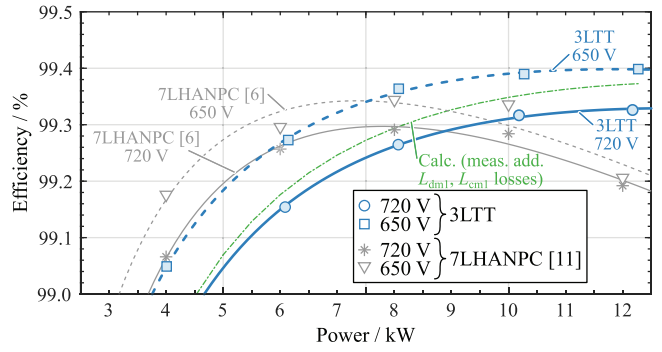
Fig. 5 Calorimetrically measured efficiencies of the 3LTT demonstrator operating with 720 V and 650 V DC input and resistive load, and calculated curve for 720 V DC (as described in [12], but using the L_{dm1} and L_{cm1} losses obtained from component-level pre-characterization). For reference, the calorimetric measurement results for the 7LHANPC prototype from [11] are shown, too.
