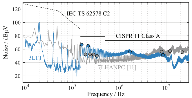
Fig. 6 Conducted EMI noise emission spectrum of the 3LTT demonstrator operating with 720 V DC. The CISPR 11 peak (PK) detector has been used with a 2 kHz step size, 9 kHz resolution bandwidth, and 10 ms measurement time for frequencies > 150 kHz, and with a resolution bandwidth of 200 Hz for frequencies < 150 kHz. In addition to the CISPR 11 Class A limit, also a proposed limit (IEC TS 62578 Class 2) for the frequency range of 9–150 kHz is indicated. Selected peaks (see markers) have been measured with the quasi-peak (QP) detector during a 1 s measurement window. For reference, we also show the measurement results for the 7LHANPC demonstrator from [11].
