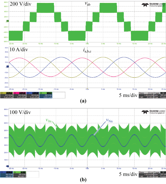
Fig. 4 Measured key waveforms of the 3LTT demonstrator operating with a 720 V DC supply and a 10 kW three-phase resistive load. (a) Switched line-to-line voltage v_{ab} and the three phase currents i_{a,b,c} . (b) HF CM voltage v_{0n} between the DC-link midpoint 0 and the negative DC rail n, and LF CM voltage v_{Nn} measured between the second-stage DM filter star point N and the negative DC rail.
