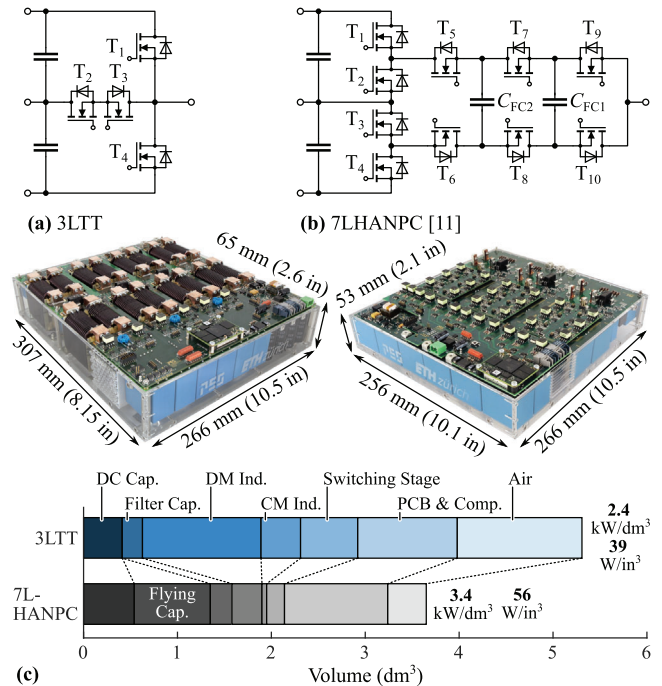
Fig. 3 12.5 kW three-phase inverter demonstrator systems realized as (a) all-SiC 3LTT inverter with DC-side CM filter (this work) and, for comparison, (b) as all-Si seven-level hybrid active-neutral-point-clamped/flying-capacitor converter (7LHANPC) [11]. (c) Volume breakdown of the two demonstrator systems. The 3LTT demonstrator's power density is 2.4 kW/dm³ (39 W/in³) and the 7LHANPC prototype's is 3.4 kW/dm³ (56 W/in³).
