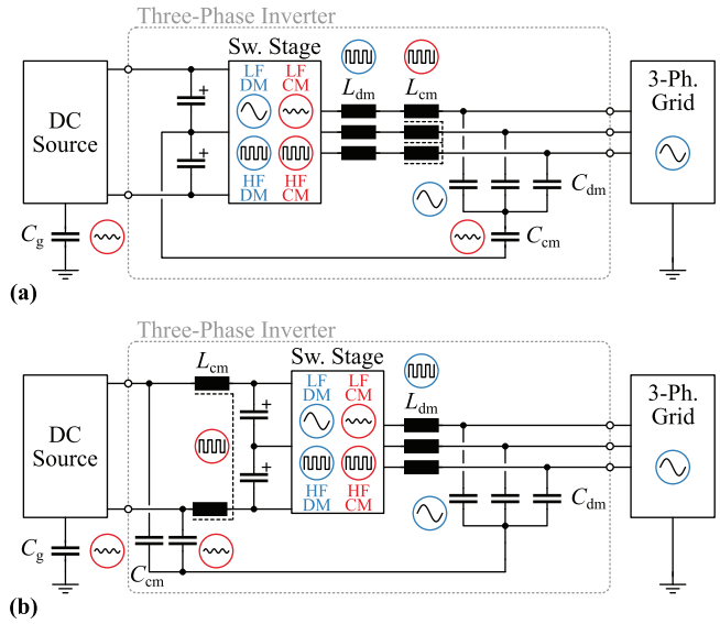
Fig. 1 Conceptual EMI filter arrangements (one filter stage shown only) for three-phase inverters for, for example, PV applications. The PWM switching stage inherently generates LF DM, HF DM, and HF CM voltages, and LF CM voltages result if third-harmonic injection is employed; these voltage components appear across the filter components and the parasitic ground capacitance C g as indicated. (a) DM and CM filter on the AC side. (b) Proposed DC-side CM filter concept and AC-side DM filter, which saves about 60% of the CM inductor's winding losses.
