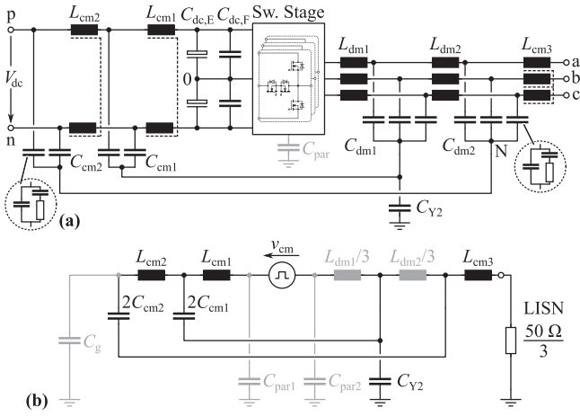
Fig. 2 (a) Power circuit of the 3LTT prototype with a DC-side CM filter. (b) CM equivalent circuit ( C_g represents the ground capacitance of the DC-side circuitry, for example, the PV panels, see Figure 1). Note that the equivalent circuit is simplified considering C_{cm} \ll C_{dm} ; even though L_{cm} \gg L_{dm} would allow a like simplification, the effective CM inductances of the DM inductors are indicated to facilitate the explanation of a potential resonance of L_{dm1}/3 with C_{par1} and C_{Y2} .
