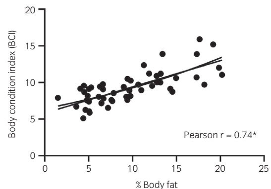
FIGURE 1 Correlation between BCI and % body fat, measured by deuterium dilution, in ponies and horses from Study 1 (University of Melbourne) from which the BCI equation was initially derived, including animals in moderate and obese body condition. The data points were fitted to a linear and nonlinear regression equation, and the goodness of fit assessed by the sum of the squares was very similar for the two methods (148.9 for the straight line fit vs. 149.8 for the curve). The Pearson r correlation value was 0.74 ( P < 0.0001 ).
