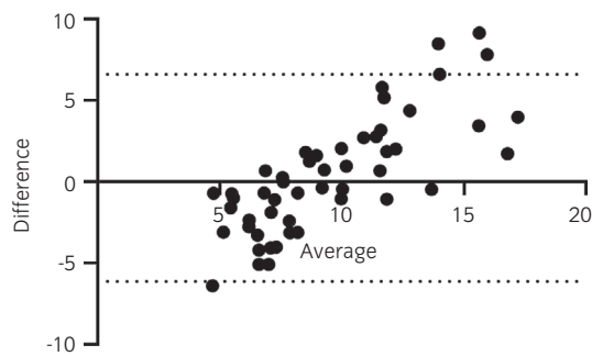
FIGURE 2 Bland-Altman plot comparing body fat assessed by deuterium dilution and estimated by the BCI method, in ponies and horses from Study 1 (University of Melbourne) from which the BCI equation was initially derived, including animals in moderate and obese body condition. The bias was 0.23 ( \pm SD 3.25), however the 95% limits of agreement (dotted lines) ranged from -6.14 to 6.60 , and the plot indicated that the BCI over-estimates the % body fat in leaner animals and under-estimates the % body fat in more obese animals.
