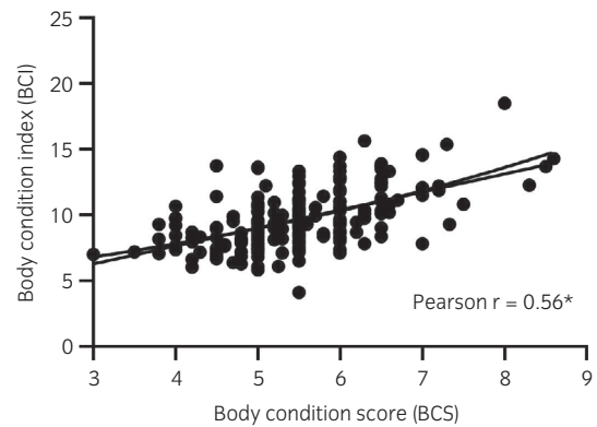
FIGURE 5 Correlation between BCI and BCS in horse breeds from Studies 3–5. The data points were fitted to a linear and nonlinear regression equation, and the goodness of fit assessed by the sum of the squares was not significantly different comparing the nonlinear equation (694) with the straight line fit (702). The Pearson r correlation value was 0.56 ( P < 0.0001 ).
