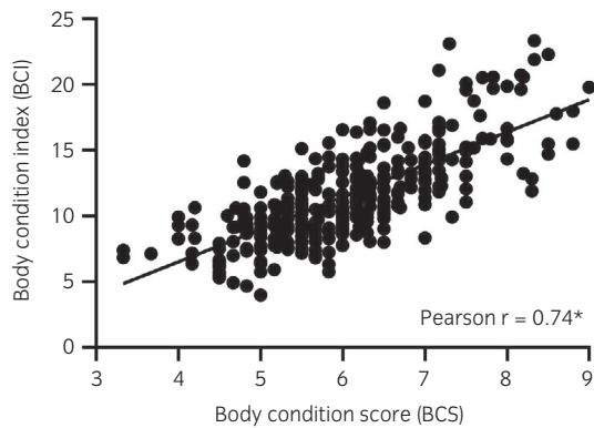
FIGURE 4 Correlation between BCI and BCS in pony breeds (excluding Shetlands and miniature ponies) from Studies 3–5. The data points were fitted to a linear and nonlinear regression equation, and the goodness of fit assessed by the sum of the squares was not significantly different comparing the nonlinear equation (1836) with the straight line fit (1861). The Pearson r correlation value was 0.74 ( P < 0.0001 ).
