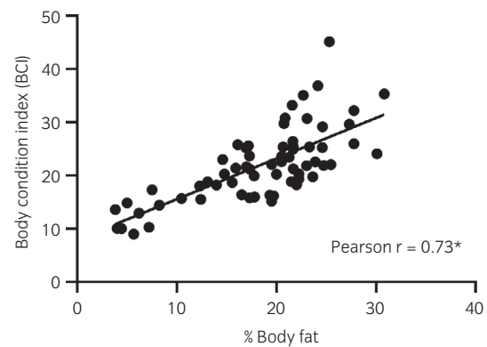
FIGURE 3 Correlation between BCI and % body fat, measured by deuterium dilution, in ponies and horses from Study 2 (SRUC) from which the BCI equation was subsequently validated, including animals in moderate and obese body condition. The data points were fitted to a linear and nonlinear regression equation, and the goodness of fit assessed by the sum of the squares was very similar for the two methods (1459 for the straight line fit vs. 1477 for the curve). The Pearson r correlation value was 0.73 ( P < 0.0001 ).
