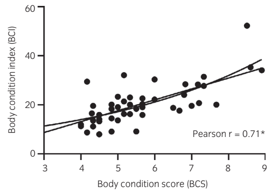
FIGURE 6 Correlation between BCI and BCS in Shetland and miniature pony breeds from Studies 3–5. The data points were fitted to a linear and nonlinear regression equation, and the goodness of fit assessed by the sum of the squares was not significantly different comparing the nonlinear equation (1538) with the straight line fit (1624). The Pearson r correlation value was 0.71 ( P < 0.0001 ).
