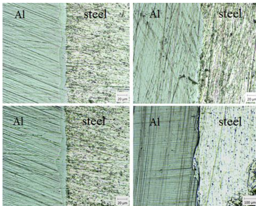
Figure 7. Microstructure in the zone of the welded joint.
