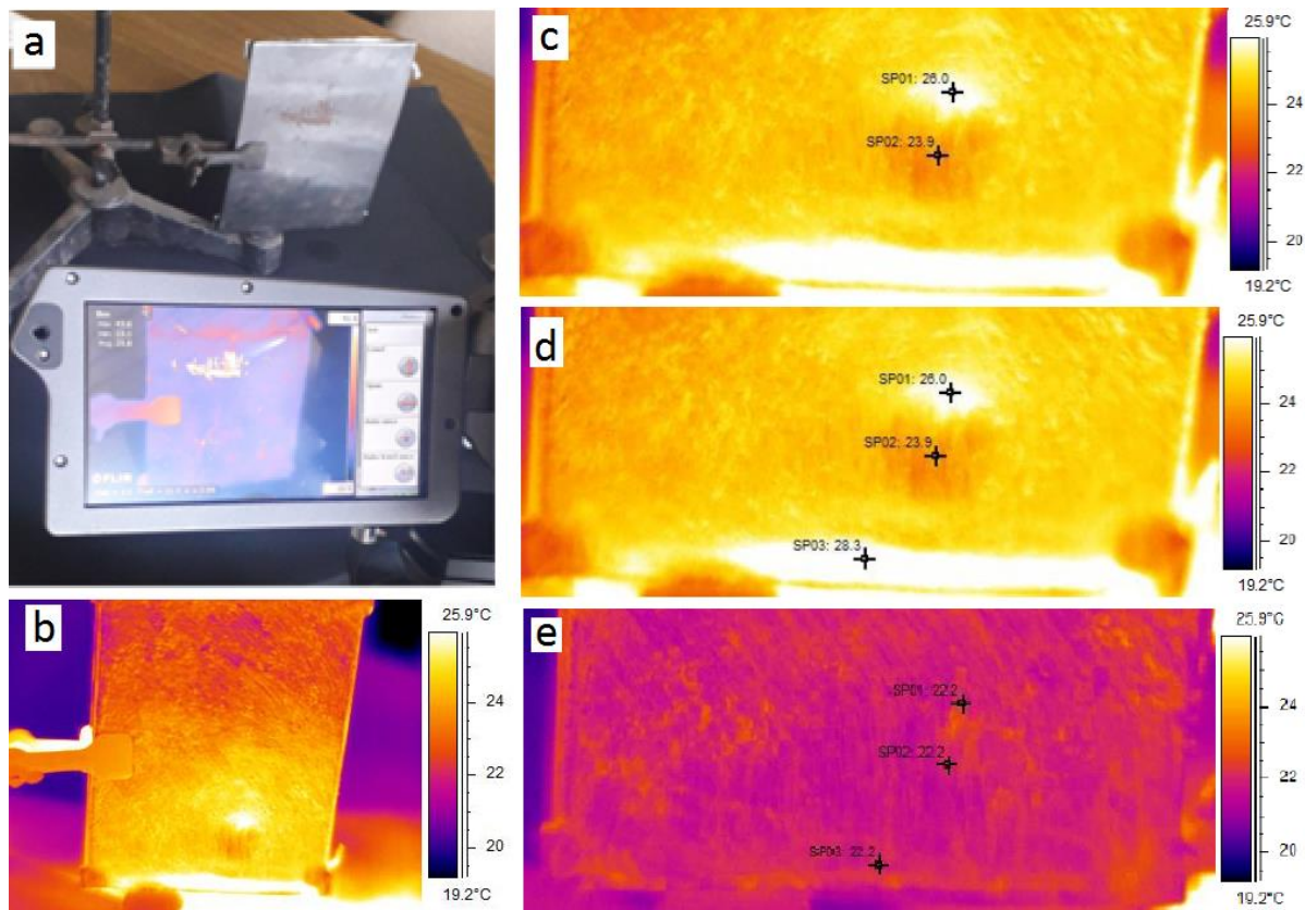
Figure 5. IR imaging results - aluminium side, heated with hot air.
