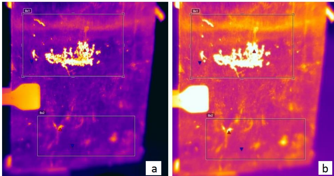
Figure 6. IR imaging results - thermogram of the steel side with marked measuring areas Bx1 and Bx2.
