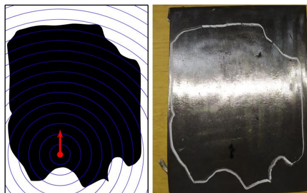
Figure 4. Zone of the weld detected by ultrasonic defectoscopy.
