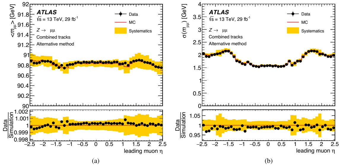
Fig. 15 a Fitted mean mass of the dimuon system for CB muons for Z \rightarrow \mu\mu events data and corrected simulation as a function of the pseudorapidity of the highest- p_T muon. b Dimuon invariant mass resolution for CB muons for Z \rightarrow \mu\mu events for data and corrected simulation as a function of the pseudorapidity of the highest- p_T muon. The upper panels show the results obtained on data and simulation after all correc-
