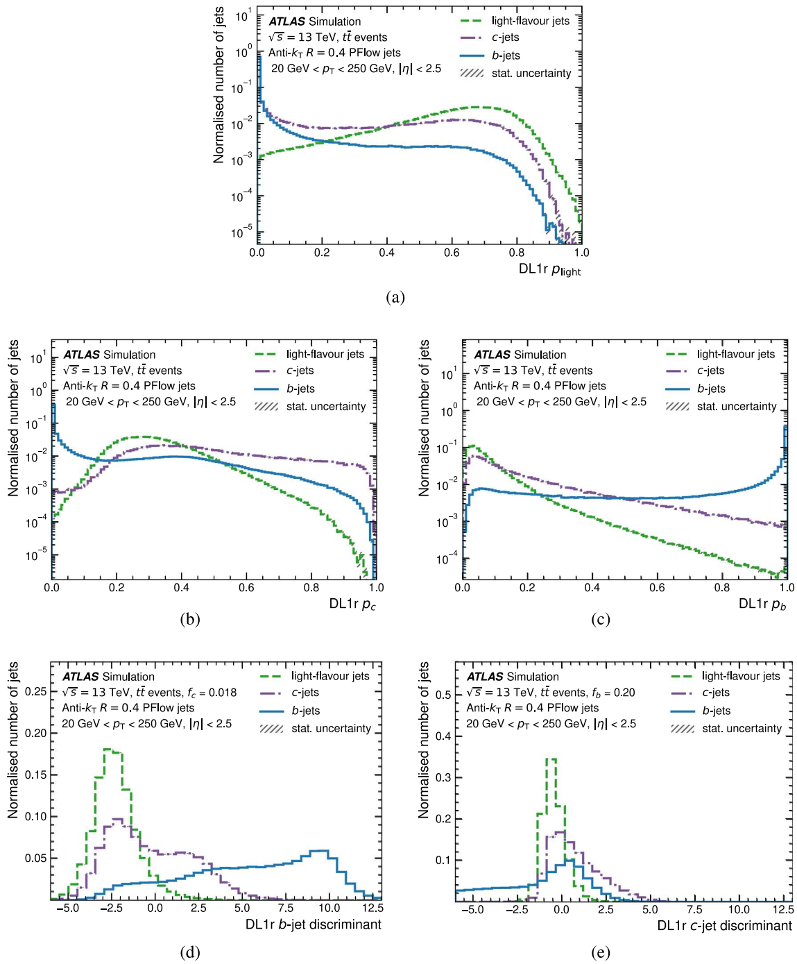
Fig. 7 Distributions of the outputs of the DL1r b -tagging algorithm for b -jets, c -jets and light-flavour jets in t\bar{t} simulated events: a p_{light} , b p_c , c p_b , d D_{DL1r} , and e D_{DL1r}^c
