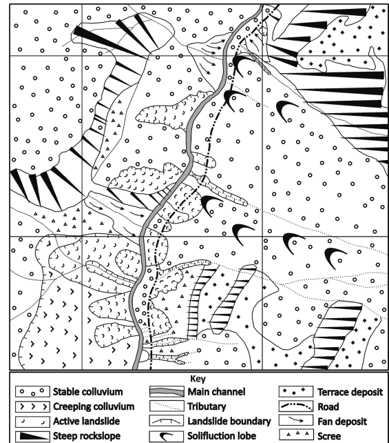
FIGURE 6.3. A terrain map used to identify the locations of existing landslides along the Arniko Highway in Nepal. The grid squares are 1 km.
