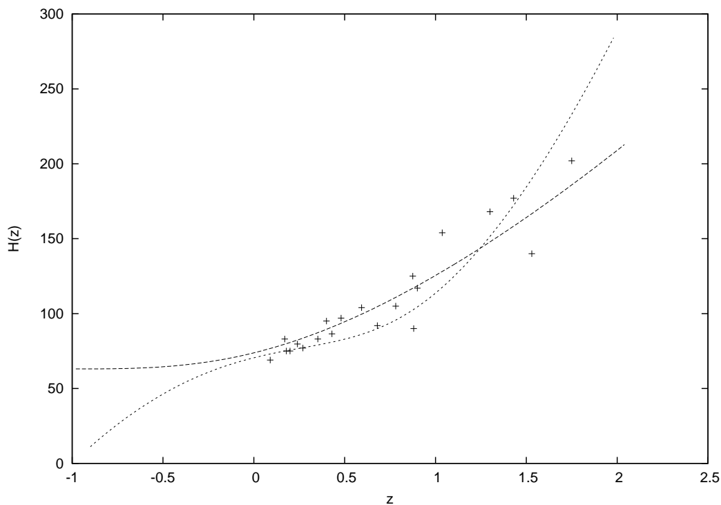
Figure 1. Comparison of experimental data from [38,40,41] for H(z) measured in units of \text{km s}^{-1} \text{Mpc}^{-1} with our predictions for z_t = 0.71 , q_0 = -0.57 and H_0 = 70.5 (dotted line) and a \Lambda CDM fit for H_0 = 73.8 and \Omega_{m,0} = 0.27 taken from [31] (dashed line).
