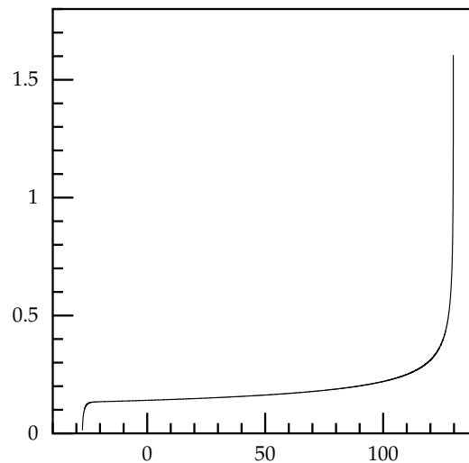
Figure 7. Global behaviour of the rotational velocity v(r) for b = b_c plotted as a function of x = \log r .
