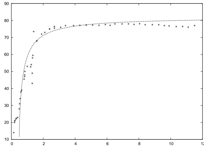
Figure 7. Global behaviour of the rotational velocity v(r) for b = b_c plotted as a function of x = \log r .
