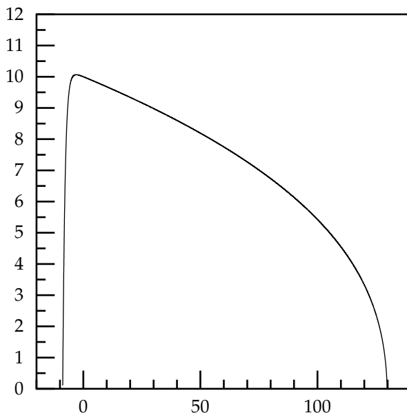
Figure 2. Numerical solution of Equation (232) for a = 10 and b = -0.03 .
