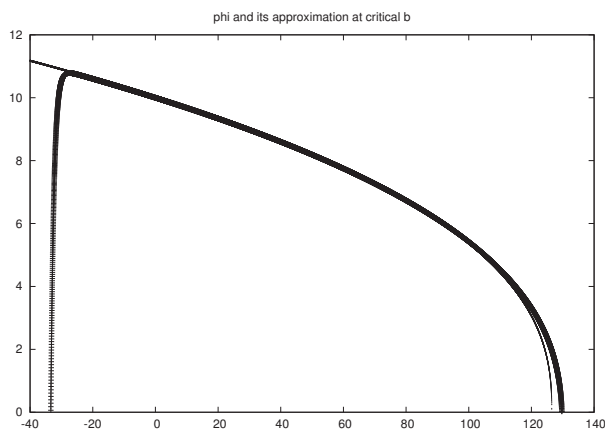
Figure 3. Numerical solution of Equaiton (232) for a = 10 and b = b_c (thick line) compared with our approximation Equaiton (243) (thin line).
