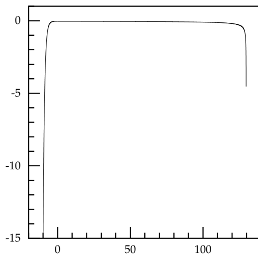
Figure 5. Numerically obtained \varphi' for a = 10 and b = -0.032 .
