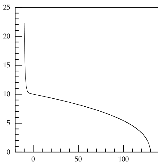
Figure 4. Numerical solution of (232) for a = 10 and b = -0.032 .
