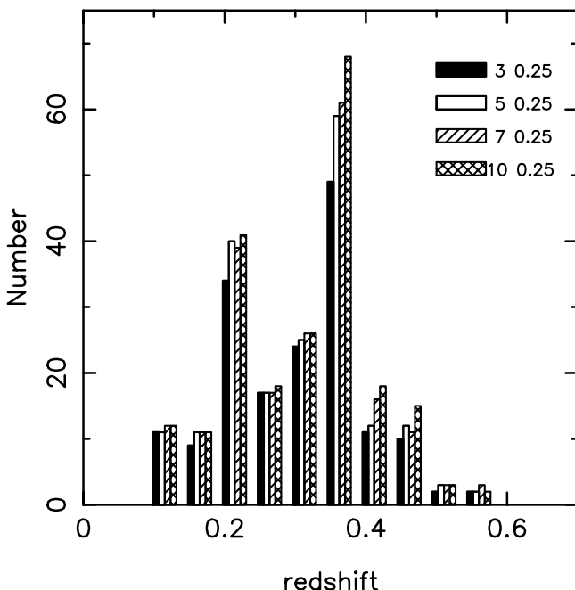
FIG. 2.—Redshift distribution of groups found with r_p^{\max} fixed at 0.25 h^{-1} Mpc and r_z^{\max} (upper right) varying over the same range as Fig. 1.
