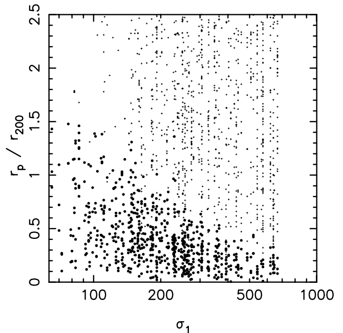
FIG. 8.—Scaled radius vs. the source group's velocity dispersion, using \Delta v^{\max} = 3\sigma_1 . The small plus signs are for all galaxies contributing to \xi_{Gg} , whereas the filled octagons mark the galaxies identified as group members.
