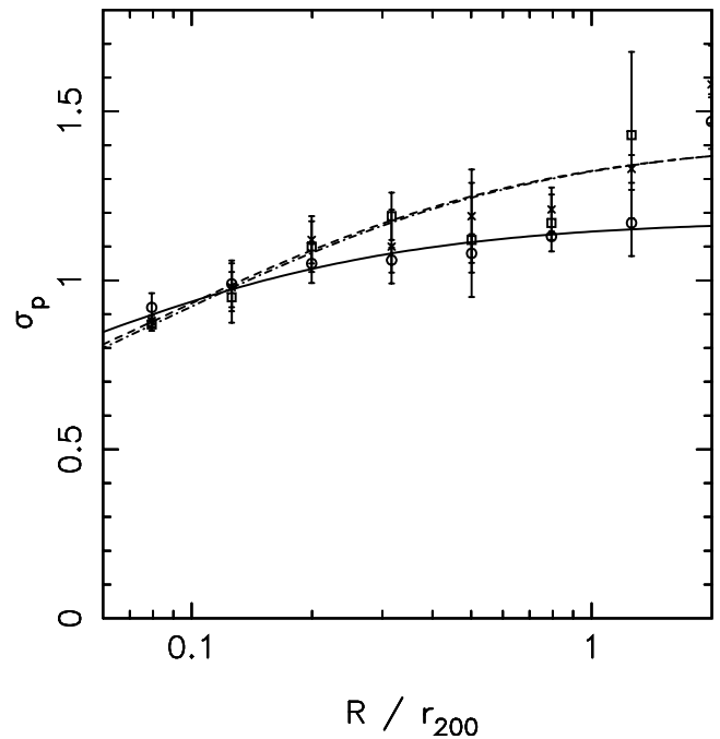
FIG. 10.—Number-weighted projected velocity dispersion profile. The circles, crosses, and squares are for velocity cuts at 3, 4, and 5 velocity unit cutoff, which are fitted by the solid, dashed, and dotted lines (virtually on top of each other).
