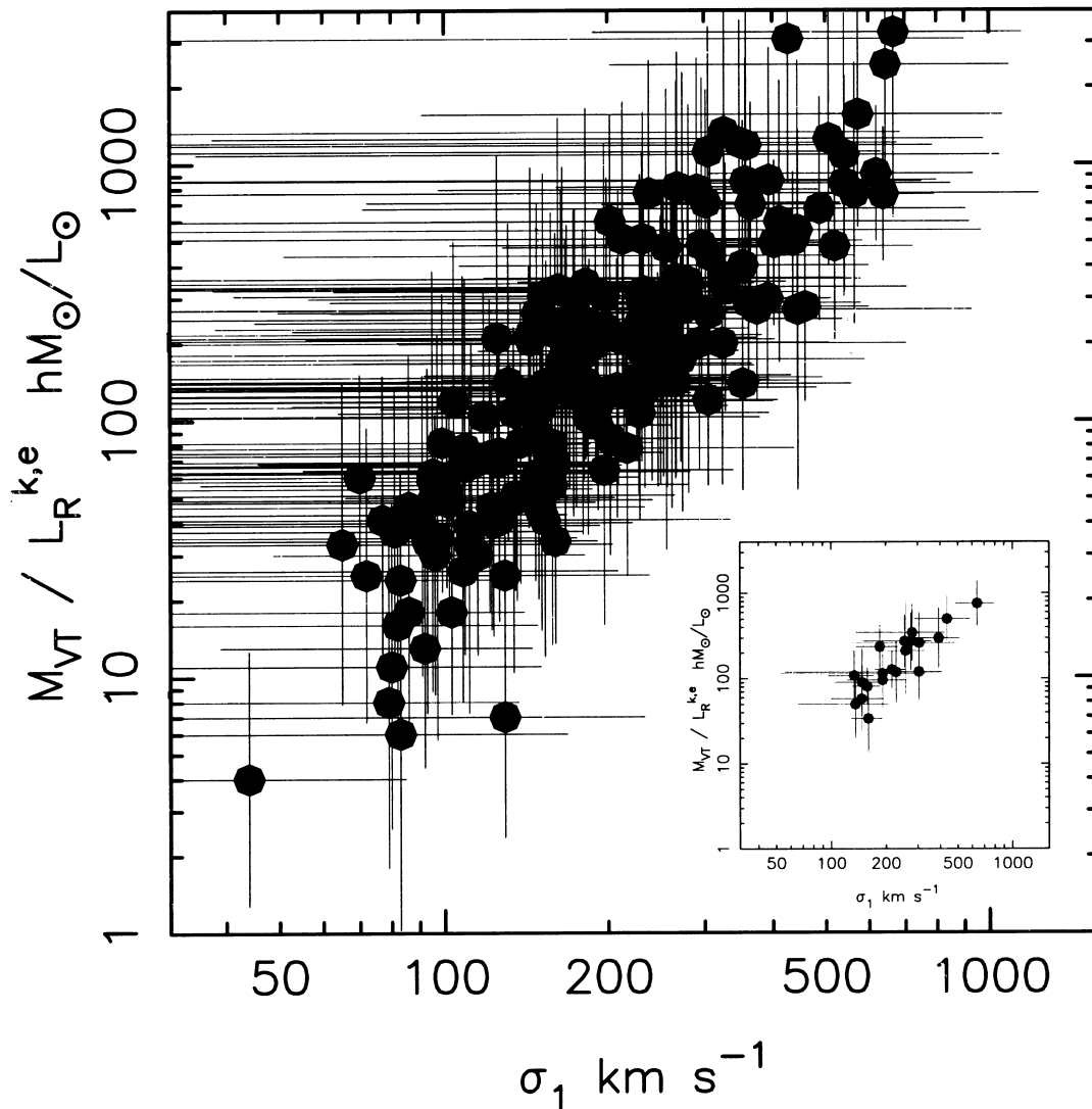
FIG. 4.—Mass-to-light ratios of the groups as a function of their velocity dispersions for r_p^{\max} = 0.25 h^{-1} Mpc and r_z^{\max} = 5 h^{-1} Mpc. The 1 \sigma error flags plotted are jackknife technique estimates. The correlation is the result of the \sigma_1^2 dependence of M_{VT} . The inset restricts the sample to groups with six or more members.
