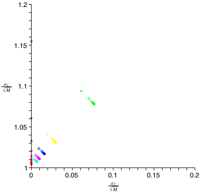
FIG. 1 (color online). The values of the dimensionless quantities a_2/\sqrt{M}, a_1/\sqrt{M} for which smooth solitons are obtained are indicated by points. The highest point on the figure corresponds to m = 2, n = 0 . Increasing n moves diagonally downwards towards the diagonal, and increasing m - n moves down towards (0, 1) . For each point, there is a set of orbifolds labeled by k . Solutions with event horizons exist in the region a_1/\sqrt{M} + a_2/\sqrt{M} < 1 (off the bottom of the plotted region).
