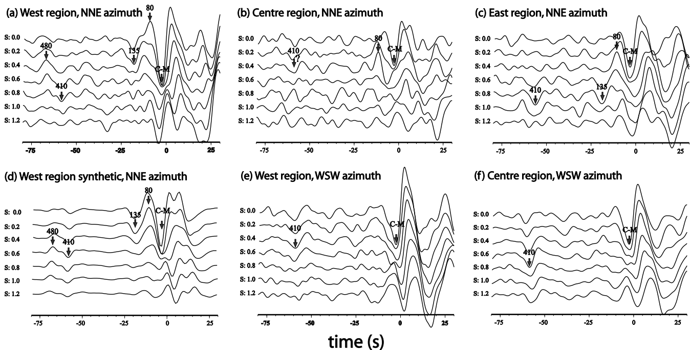
Figure 2. Stacked S receiver functions characterizing different regions and directions of wave propagation: (a) western region, NNE backazimuth, 100 recordings; (b) central region, NNE backazimuth, 65 recordings; (c) eastern region, NNE backazimuth, 78 recordings; (d) synthetic stack for the western region, NNE backazimuth; (e) western region, WSW backazimuth, 65 recordings; (f) central region, WSW backazimuth, 105 recordings. The S velocity model used to generate the synthetic stack in (d) is shown in Fig. 3 (Iceland). The numbers from 0.0 to 1.2 are differential slowness for the corresponding traces in \text{s deg}^{-1} . Arrows indicate seismic arrivals discussed in the text and the corresponding numbers indicate the depths deduced for the related discontinuities. The arrows point to the traces with the largest amplitudes. C–M denotes the crust–mantle boundary. Because the piercing points are displaced from the receivers in the directions of the epicentres of the seismic events, the S_p phases from the events from the WSW at the eastern stations mostly characterize the upper mantle not of the eastern but of the central region. For this reason, the stack for the eastern region is not shown.
