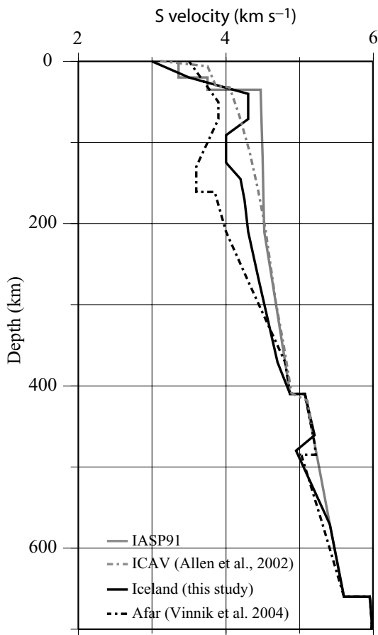
Figure 3. S velocity models: Iceland, the best-fitting model for the western region using synthetic modelling of the data from the NNE backazimuth (Figs 2a and d); Afar, the best-fitting model for the mantle beneath the Afro-Arabian hotspot (Vinnik et al. 2004); ICAV, the model derived from average phase velocity of surface Love waves across Iceland (Allen et al. 2002); IASP91, the IASP91 global model (Kennett & Engdahl 1991).
