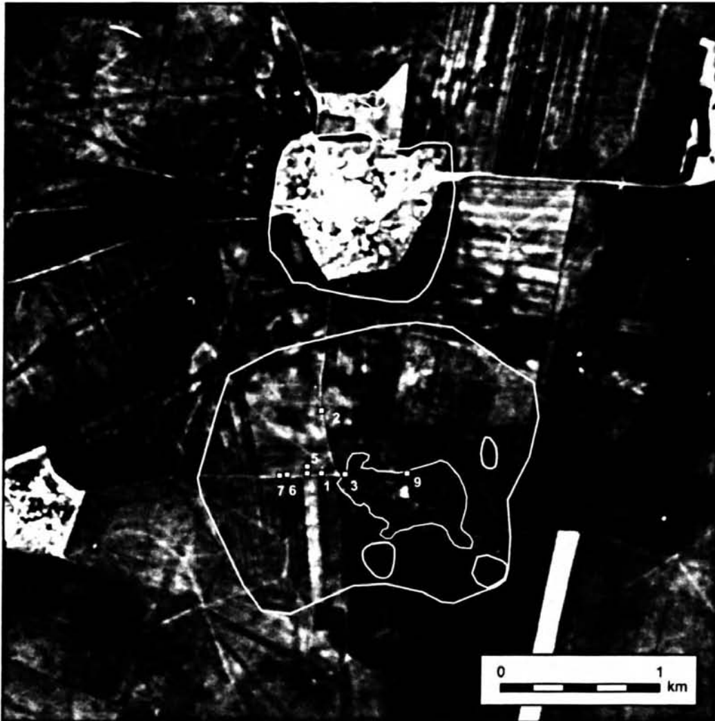
Fig. 5. CORONA image of the Hamoukar southern extension showing the location of Trenches Z 1-7 and Z 9.
