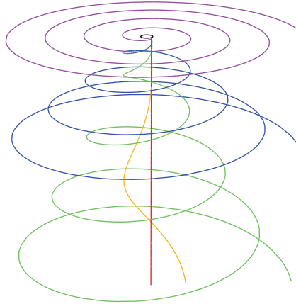
Figure 3: The spiral string solution in AdS_5 spacetime corresponding to quark undergoing a circular motion. The curves are drawn for differing values of the quark velocity v on the boundary (values of v and color-coding are the same as in Figure 2). The small black circle on the top is the quark trajectory on the AdS boundary; the vertical direction corresponds to the bulk radial direction.
