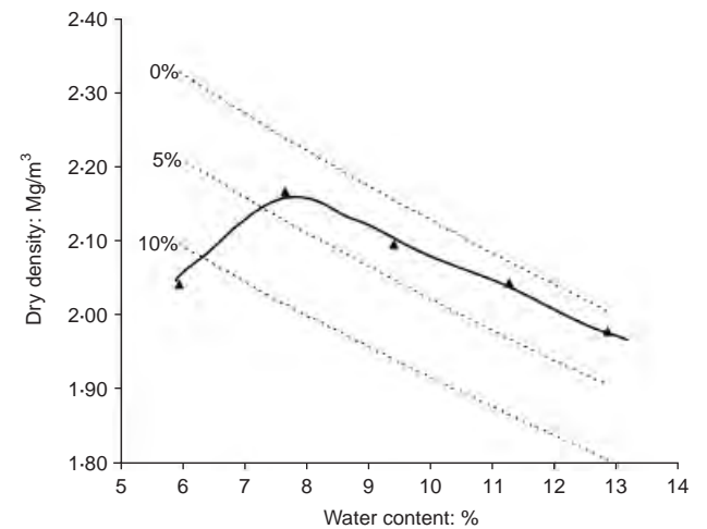
Fig. 3. Compaction curve from vibrating hammer test. Dotted lines correspond to different proportions of pore air volume
