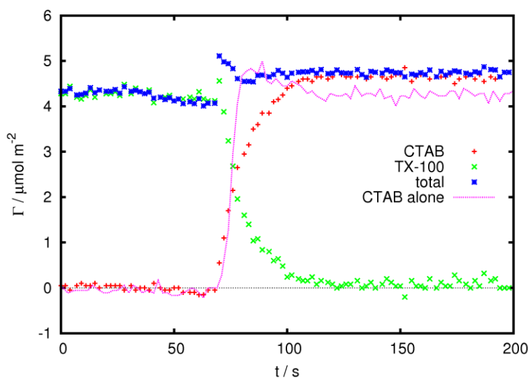
Figure 9: Replacement of 2 mM TX-100 (green ×) with 2 mM CTAB (red +). The total surface excess is shown as blue stars. The adsorption of 2 mM CTAB onto a clean silica surface (line) is shown for comparison.
