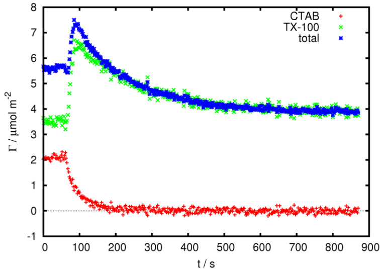
Figure 12: Replacement of a 2-mM mixed surfactant solution with \chi_{\text{CTAB}} = 0.5 by 2-mM TX-100. Adsorbed amounts: CTAB (+, red), TX-100 (x, green), total (*, blue).
