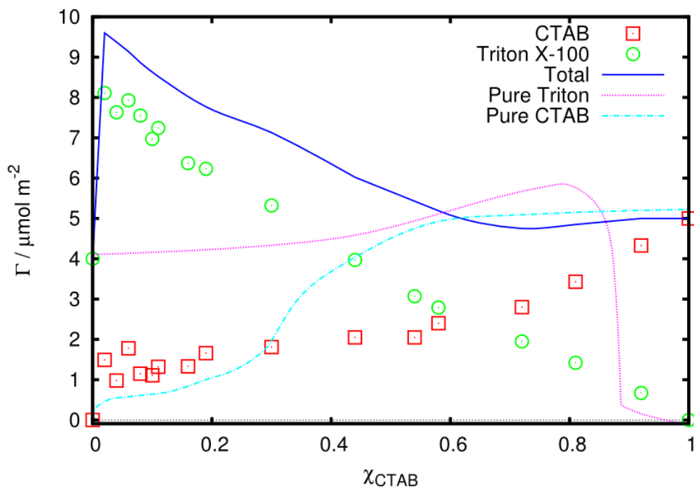
Figure 5: Surface excess of CTAB (squares) and TX-100 (circles) at a total surfactant concentration of 2 mM as a function of the bulk mole fraction of CTAB, \chi_{CTAB} , together with the total surface excess (solid line). The isotherms for the pure components at the same concentrations as that component in the mixture are indicated with dotted lines.
