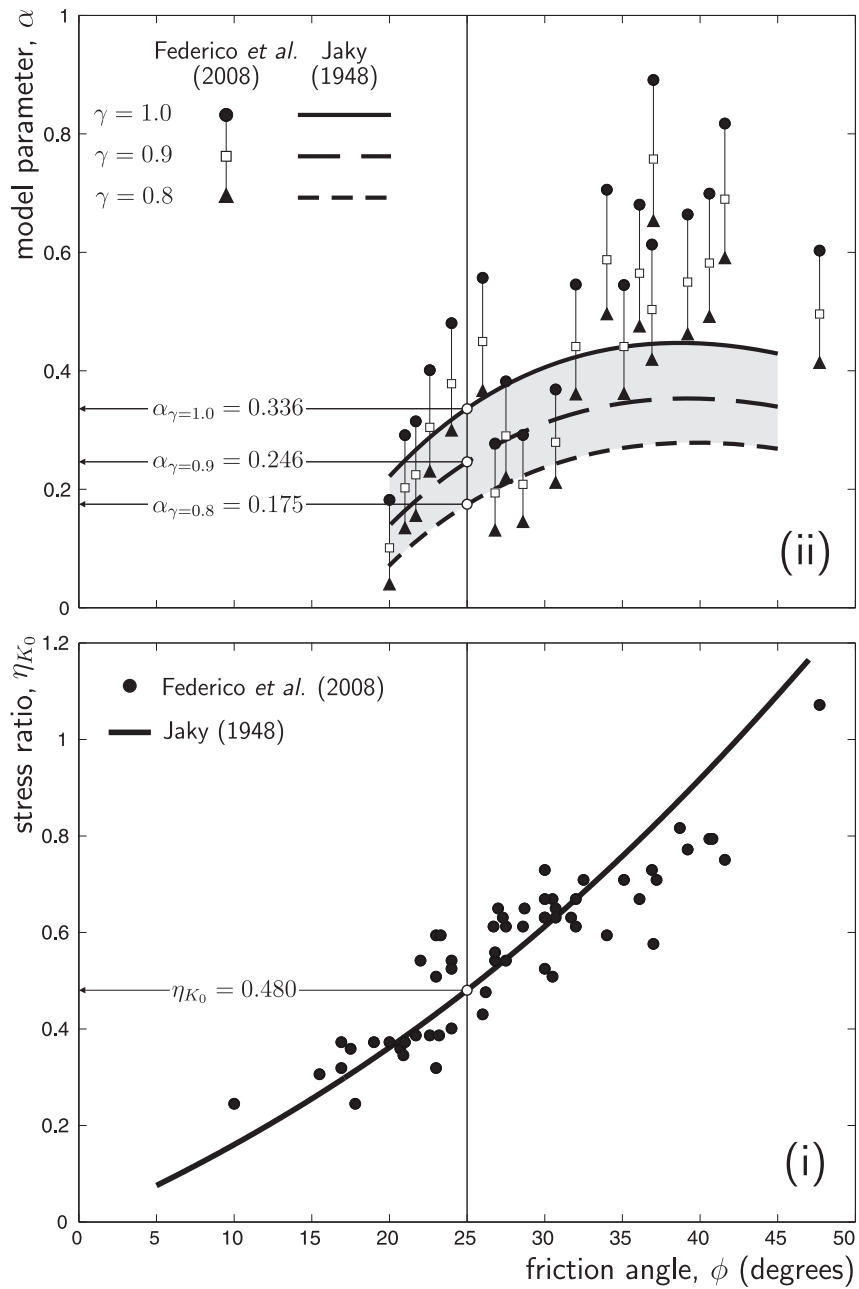
Figure 9: Calibration of material constant \alpha : (i) one-dimensional consolidation stress ratio against friction angle, comparing experimental data (discrete points) [19] against Jaky's equation [30] and (ii) \alpha ranges for \gamma = 0.8, 0.9 and 1.0 , corresponding to the data obtained from [19]. Graph (ii) also shows the \alpha versus friction angle relationships for \gamma = 0.8, 0.9 and 1.0 using Jaky's [30] relationship.
