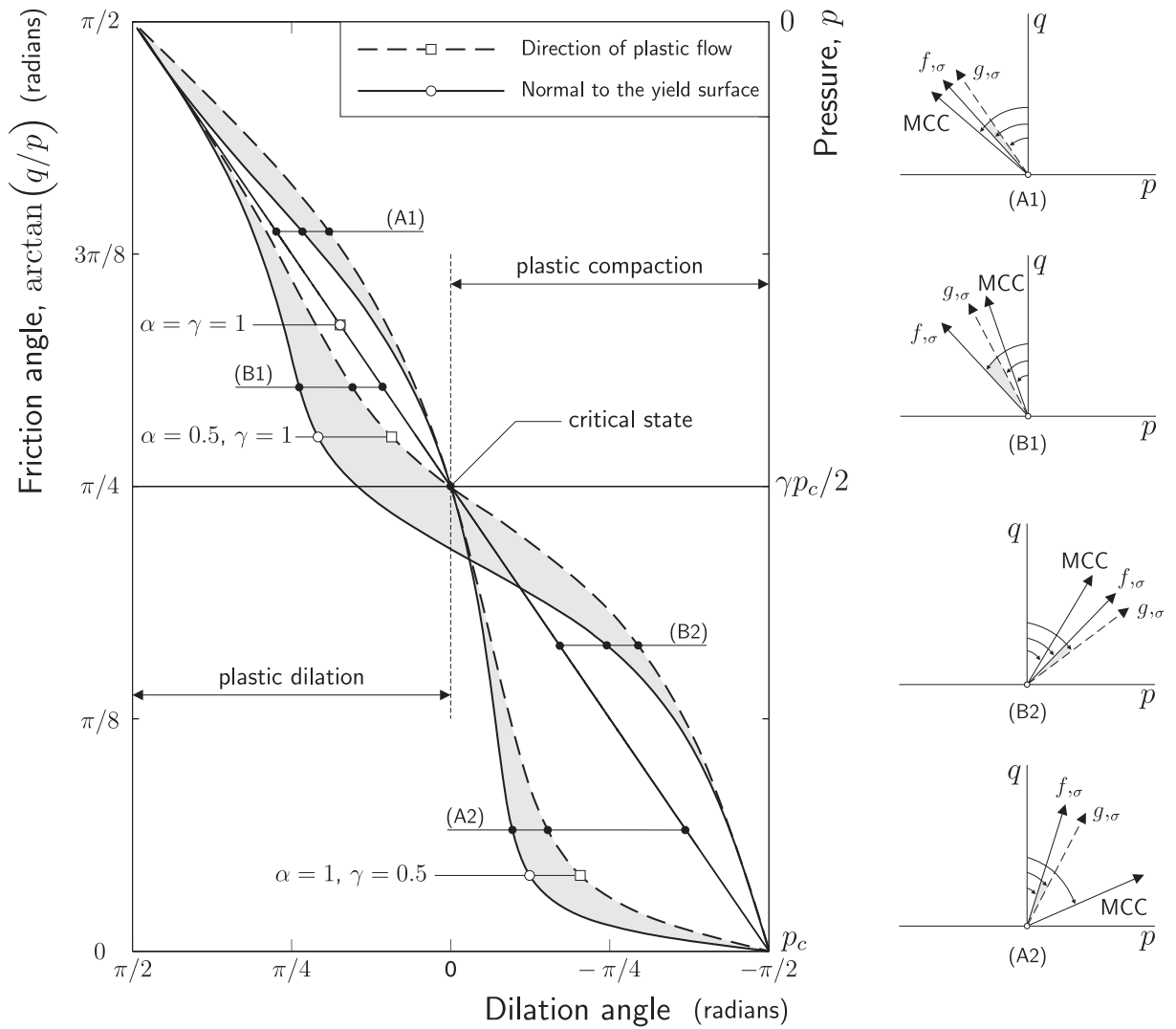
Figure 10: Dilation angle for the plastic flow direction and the normal to the yield surface for \alpha = \gamma = 1 , \alpha = 0.5, \gamma = 1 (B1-2) and \alpha = 1, \gamma = 0.5 (A1-2). The width of the shaded region indicates the degree of non-associatedness of the flow.
