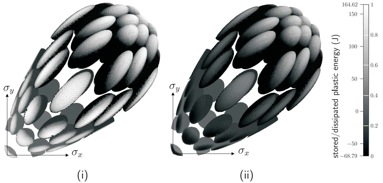
Figure 16: Three dimensional Gudehus stress plots with shading according to (i) dissipated plastic energy and (ii) stored plastic energy. The maximum and minimum work for each stress surface is identified by 1 and 0 corresponding to 164.6 J and -68.8 J, respectively.
