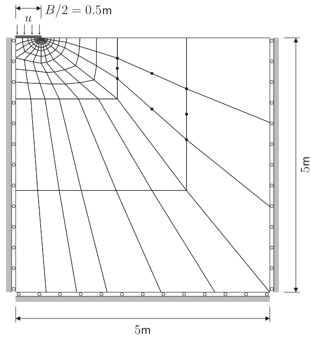
Figure 22: Rigid strip footing plane-strain finite element discretisation.
