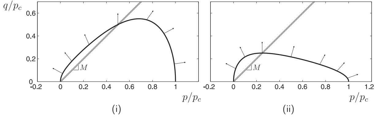
Figure 4: Yield surfaces and direction of plastic flow for the two-parameter Critical State models: (i) \alpha = 0.5 and \gamma = 1 (ii) \alpha = 1 and \gamma = 0.5 .
