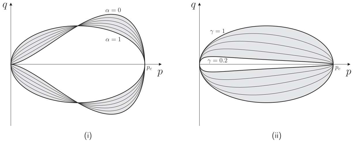
Figure 2: Yield surfaces for the two-parameter Critical State hyperplastic models: (i) \alpha \in [0, 1] with \gamma = 1 (ii) \gamma \in [0.2, 1] with \alpha = 1 .
