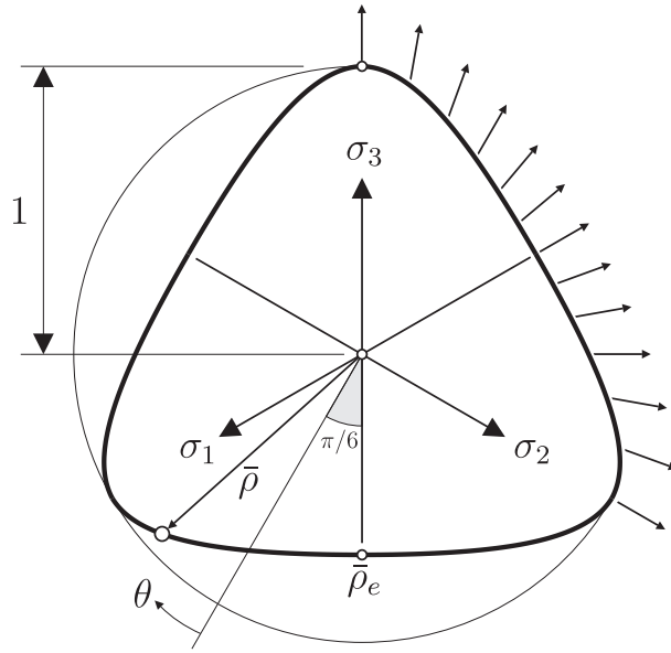
Figure 6: Willam-Warnke deviatoric section illustrating the direction of the (non-associated) radial deviatoric plastic flow.
