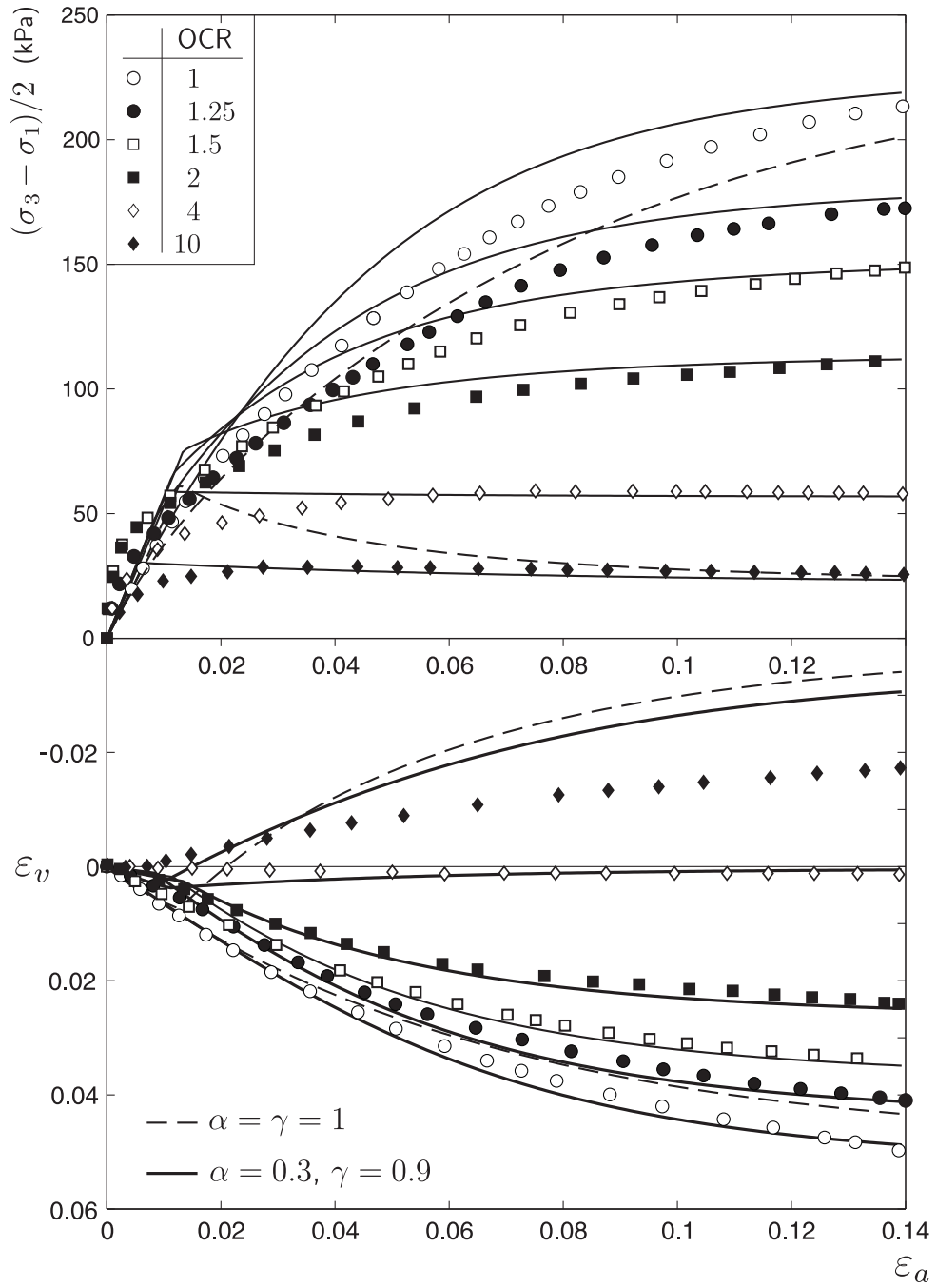
Figure 14: Drained triaxial compression test simulations compared with experimental data (shown by discrete points) [20]. Above: axial strain ( \epsilon_a ) against deviatoric stress ((\sigma_3 - \sigma_1)/2) . Below: axial strain ( \epsilon_a ) against volumetric strain ( \epsilon_v ).
