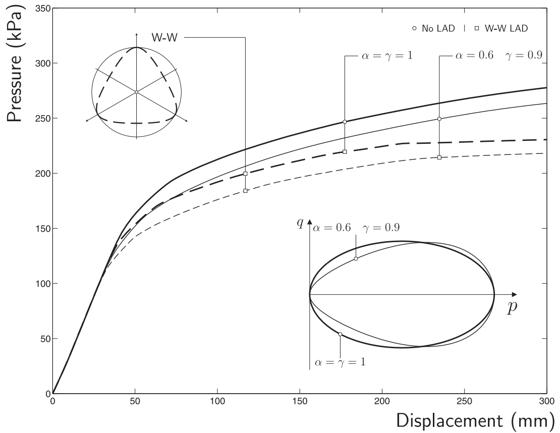
Figure 23: Rigid strip footing pressure-displacement response.
