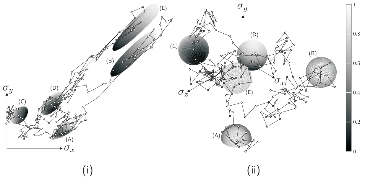
Figure 17: Sequence of Gudehus stress plots demonstrating the robustness of the BE stress return algorithm for (i) \sigma_x - \sigma_y plane and (ii) deviatoric view. The surfaces are shaded according to the length of the stress path with the maximum and minimum length identified by 1 and 0, respectively. Five of the 200 Gudehus plots are presented for steps 1 (A), 50 (B), 100 (C), 150 (D) and 200 (E).
