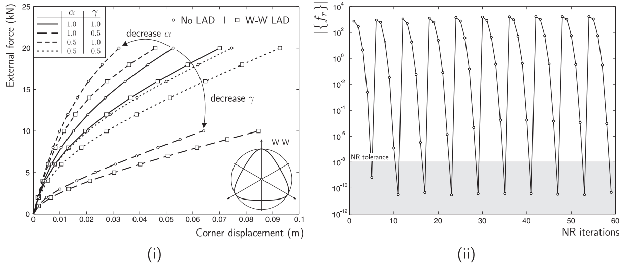
Figure 20: Single 3D finite element analysis results (i) force-displacement plots for different forms of the model, with and without LAD (ii) convergence for the W-W LAD ( \alpha = \gamma = 0.5 ).
