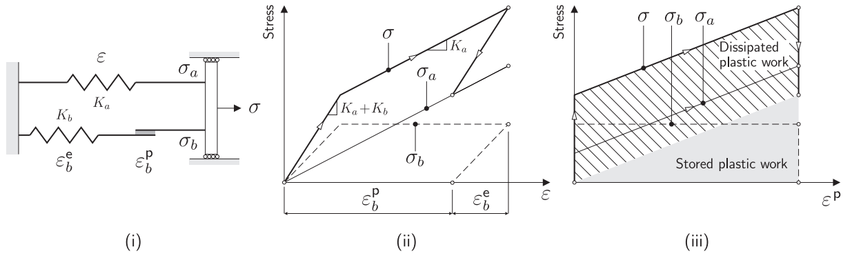
Figure 1: (i) Rheological model of a one dimensional kinematic hardening elasto-plastic system (after Collins [12]) (ii) stress-total strain response (iii) stress-plastic strain response.
