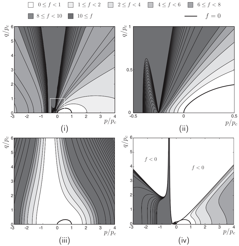
Figure 18: Contours of the yield function outside of the yield surface for a two-parameter Critical State model where \alpha = \gamma = 0.5 (i) f given by (71) from [7–9,11], (ii) local detail of f given by (71), (iii) f given by (36)_1 and (iv) f from (73) with negative regions appearing outside the yield surface.
