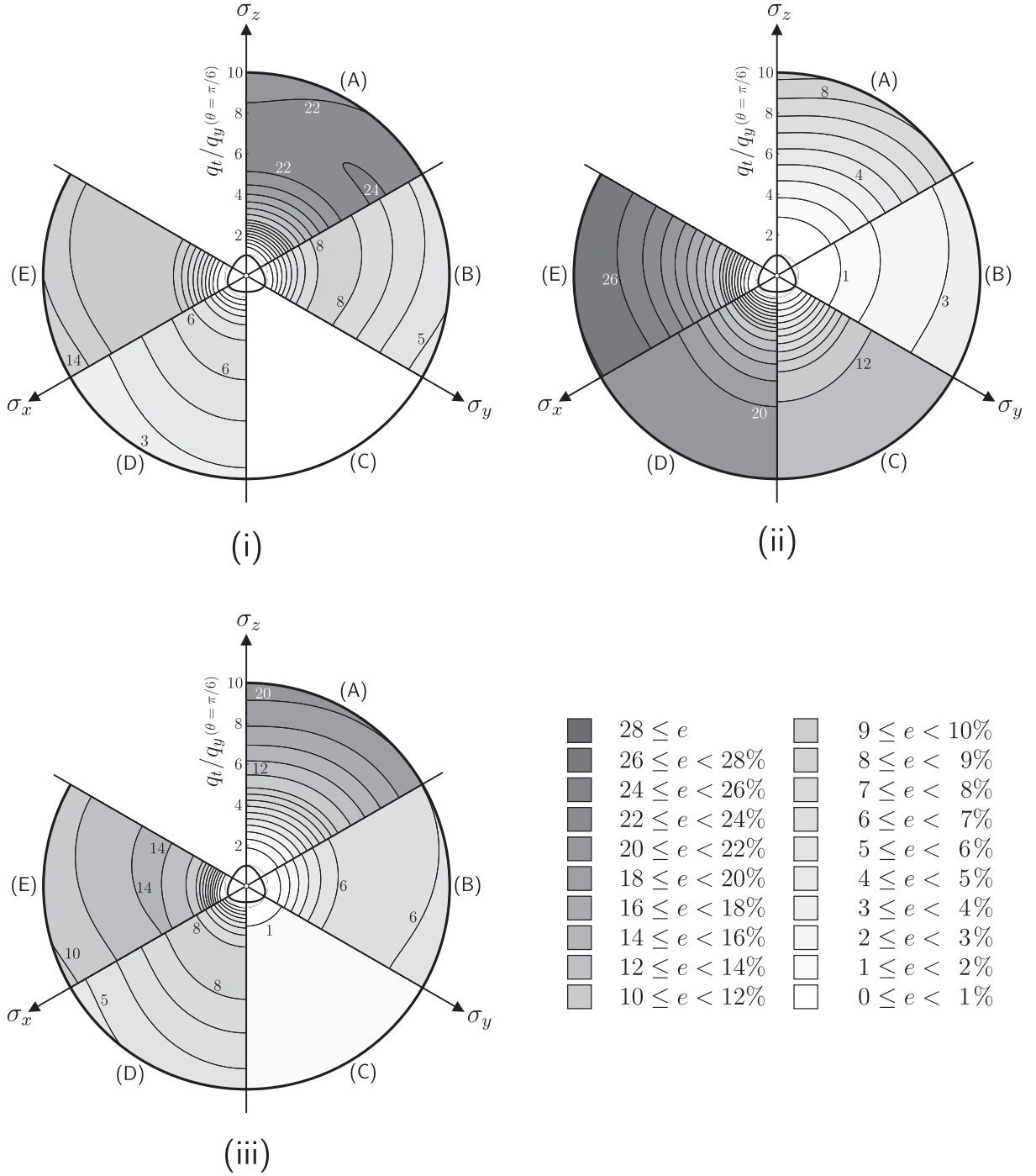
Figure 13: Errors associated with the iterative BE stress return for five pressure ratios (A) p/p_c = 0.1 , (B) p/p_c = 0.3 , (C) p/p_c = 0.5 , (D) p/p_c = 0.7 and (E) p/p_c = 0.9 for (i) \alpha = \gamma = 1 , (ii) \alpha = \gamma = 0.5 and (iii) \alpha = 0.6 , \gamma = 0.9 .
