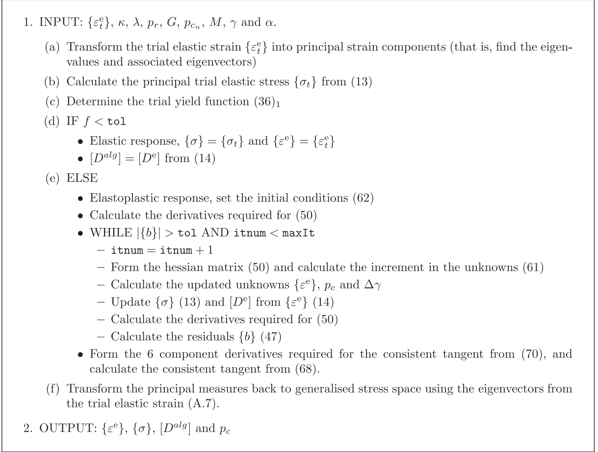
Figure 12: Pseudo code for the two-parameter family of Critical State models. The tolerance ( \text{tol} ) was typically set to 1 \times 10^{-12} .
