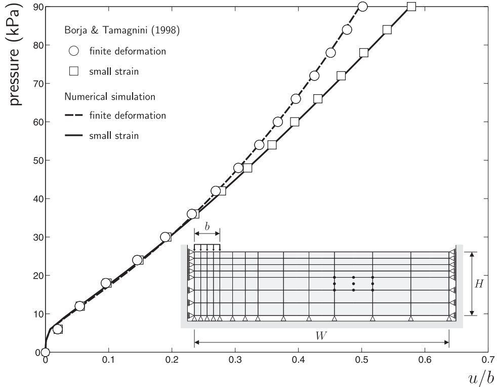
Figure 21: Flexible footing analysis: comparison between the MCC model's pressure-centreline displacement response from Borja and Tamagnini [3] (shown by discrete points) and that obtained from the analysis framework used in this paper.
