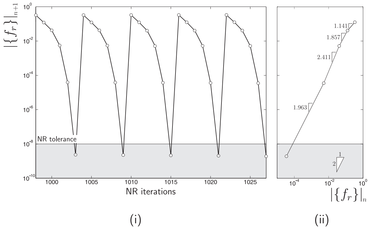
Figure 26: Convergence results for the finite deformation expansion of a cylindrical cavity when \alpha = 0.5 and \gamma = 1 with W-W LAD: (i) norm of the residual out-of-balance force for the final five loadsteps (ii) norm of the residual out-of-balance force against the previous out-of-balance force for the final loadstep.
