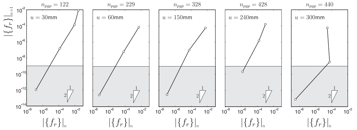
Figure 24: Rigid strip footing convergence showing the norm of the residual out-of-balance force against the previous out-of-balance force for loadsteps 10, 20, 50, 80 and 100.
