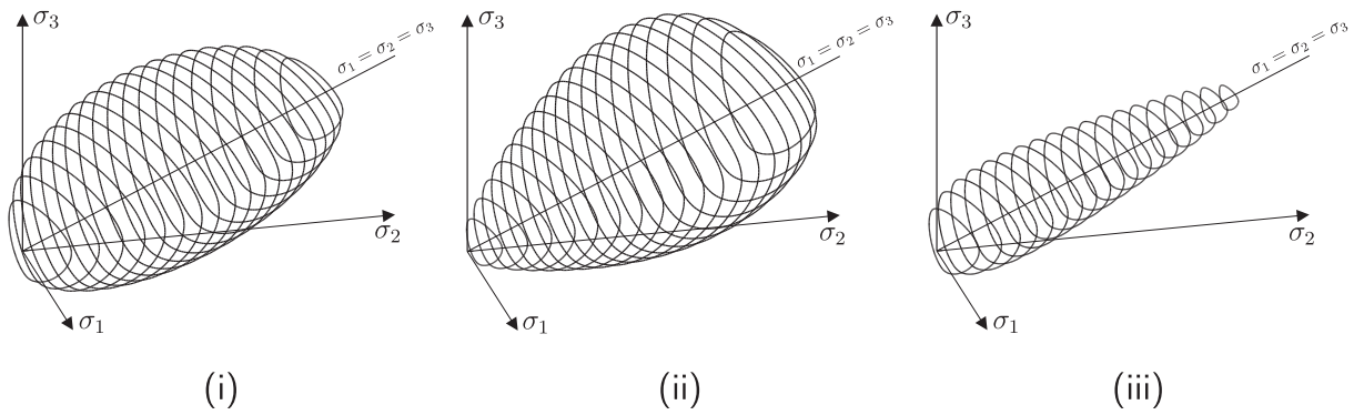
Figure 7: Two-parameter Critical State family of models with W-W deviatoric sections: (i) \alpha = \gamma = 1 , (ii) \alpha = 0.5, \gamma = 1 and (iii) \alpha = 1, \gamma = 0.5 .
