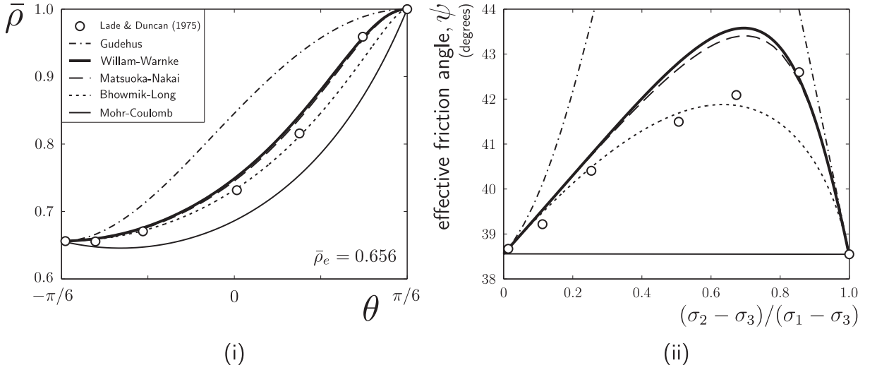
Figure 5: Comparison of Lode angle deviatoric functions with experimental data from Lade and Duncan [31] (i) deviatoric function Lode angle dependency and (ii) variation of the effective friction angle with the ratio of the intermediate principal stress.
