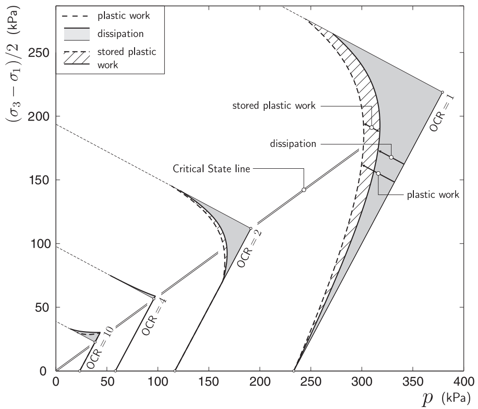
Figure 15: Drained triaxial compression stress paths showing the cumulative plastic work and dissipation for the two-parameter model with \alpha = 0.3 and \gamma = 0.9 .
