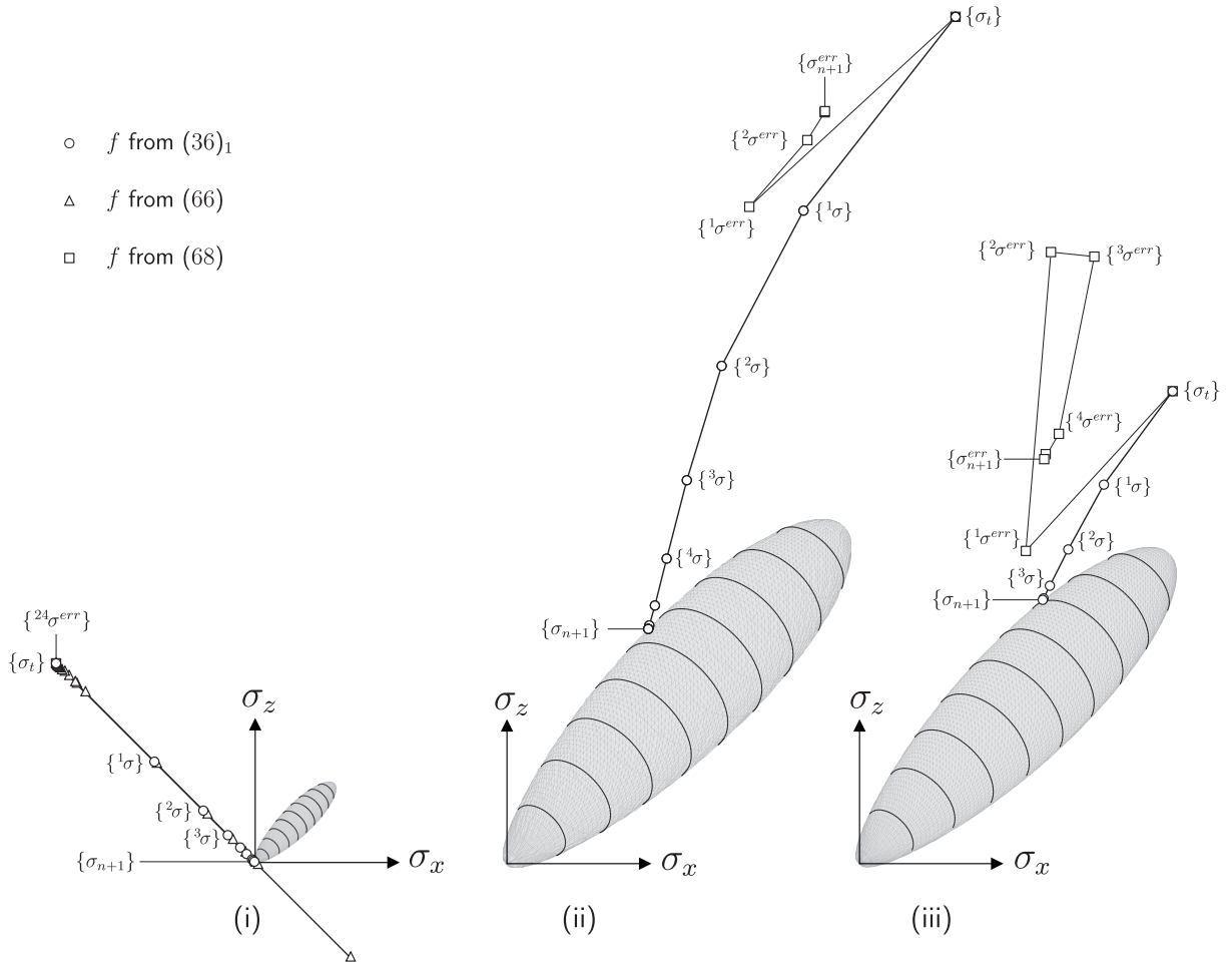
Figure 19: Stress returns (associated with yield functions (36) 1 , (71) and (73)) for three different trial states (i)-(iii).
