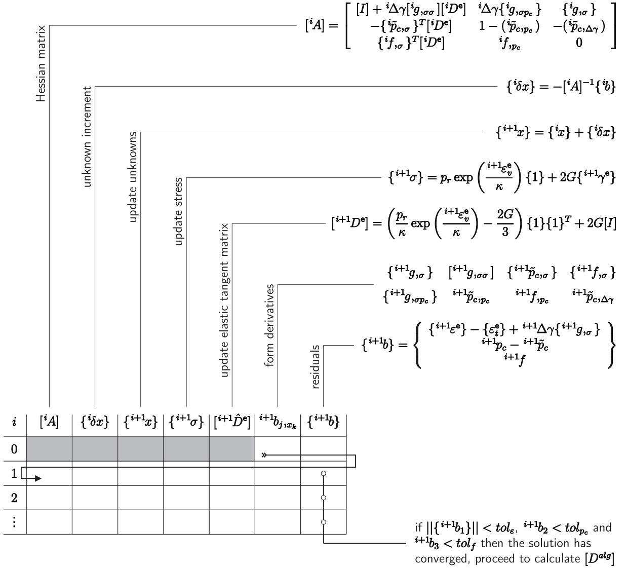
Figure 11: Backward Euler stress return sequence.
