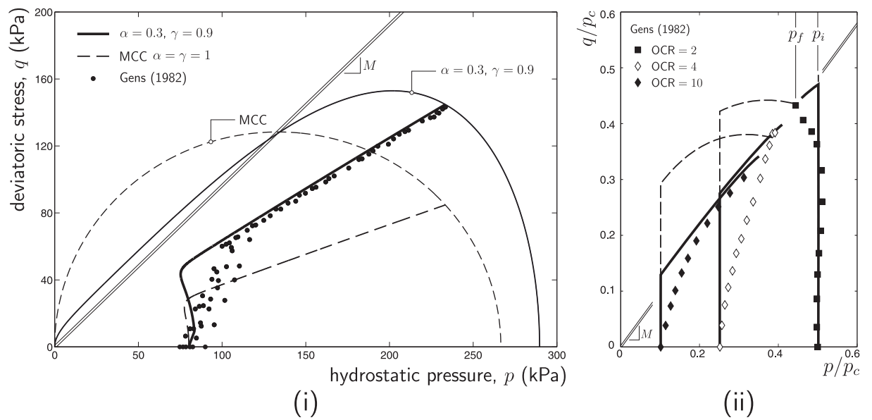
Figure 8: Test simulations using the MCC model ( \alpha = \gamma = 1 ) and the two-parameter model ( \alpha = 0.3, \gamma = 0.9 ) compared against experimental data (shown by discrete points) from Gens [20]: (i) one-dimensional consolidation (ii) undrained triaxial compression with OCR = 2, 4 and 10 (the dashed line indicates the MCC model response, whereas the continuous line shows the stress path obtained from the two-parameter hyperplastic model).
