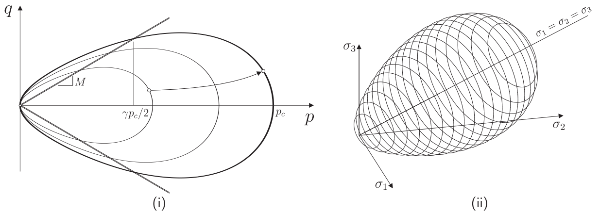
Figure 3: Yield surfaces for \alpha = 0.6 and \gamma = 0.9 with no LAD (i) p - q stress space showing isotropic hardening (ii) principal stress space.
