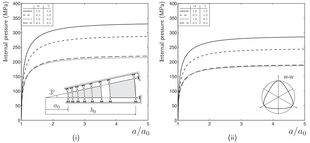
Figure 25: Finite deformation expansion of a cylindrical cavity (i) no LAD (ii) W-W LAD with \bar{p}_e = 0.7695 .
